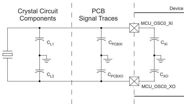
Figure 7-18. Load Capacitance
