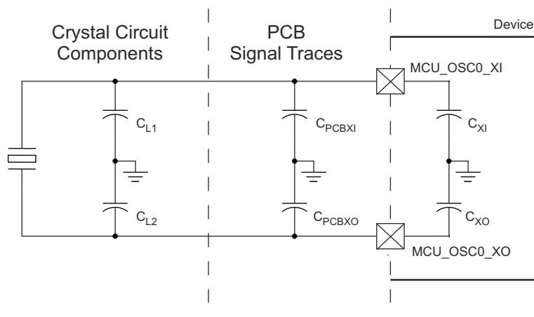
Figure 7-18. Load Capacitance
