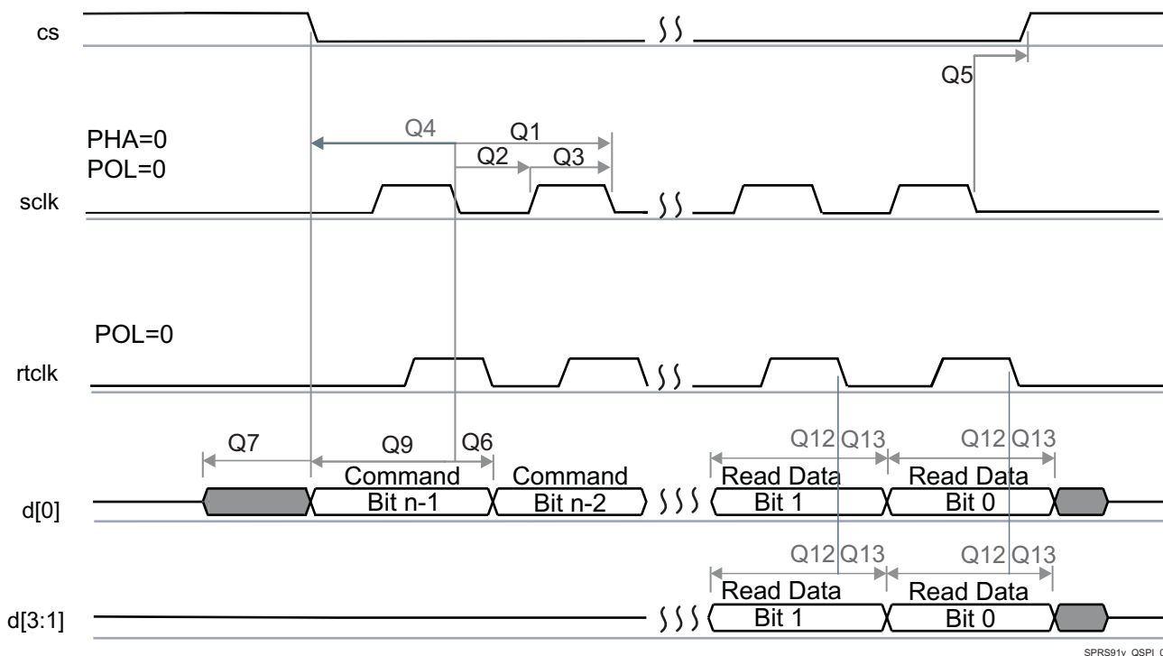
Figure 5-55. QSPI Read (Clock Mode 0)
