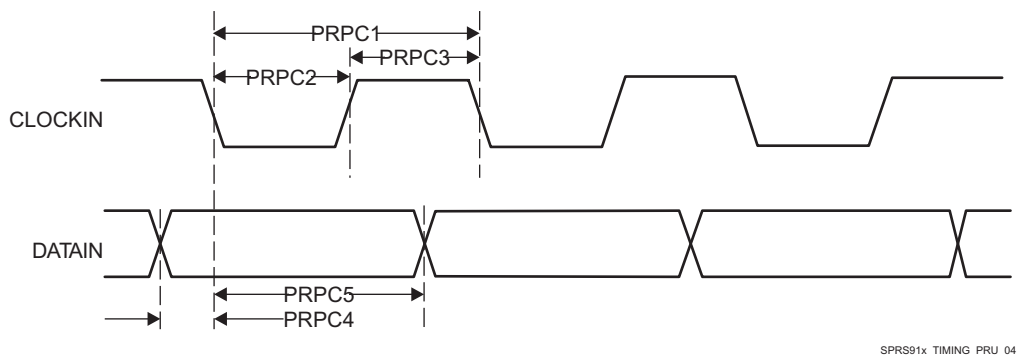
Figure 5-111. PRU-ICSS PRU Parallel Capture Timing - Falling Edge Mode
