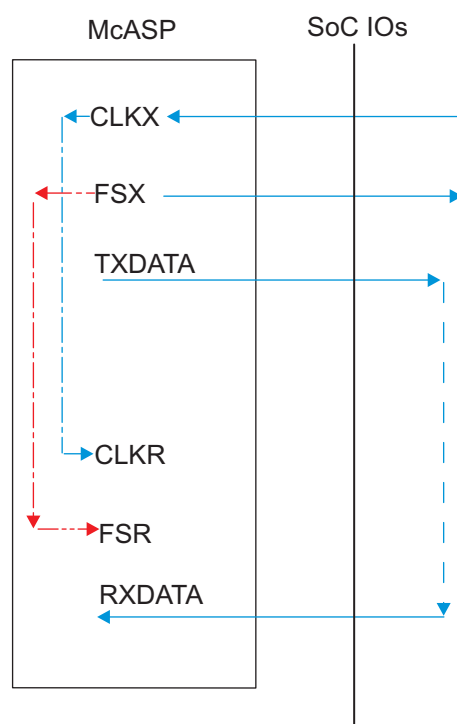
Figure 5-65. McASP1-8 CI-FO- – SYNC Mode
