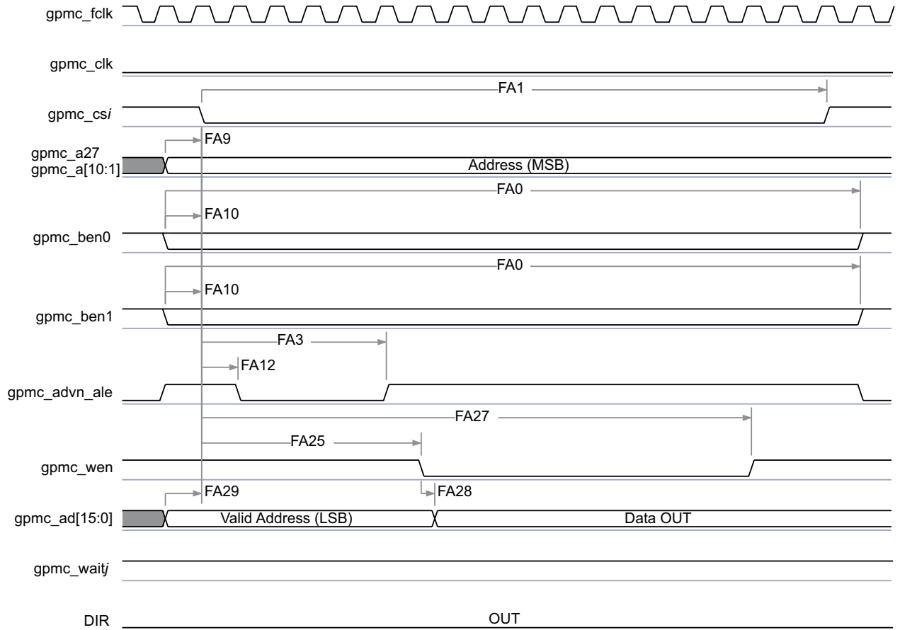
Figure 5-35. GPMC / Multiplexed NOR Flash - Asynchronous Write - Single Word Timing (1)(2)
