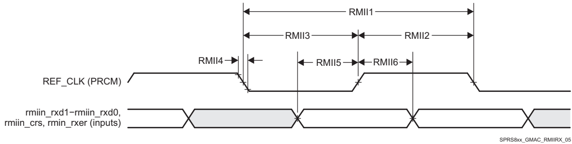
Figure 5-73. GMAC Receive Interface Timing RMIIIn Operation
