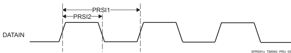
Figure 5-112. PRU-ICSS PRU Shift In Timing
