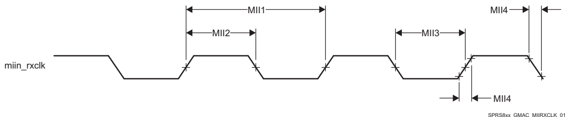
Figure 5-68. Clock Timing (GMAC Receive) - MII n operation
