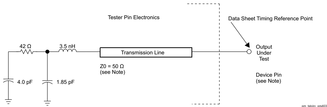
Figure 5-2. Test Load Circuit for AC Timing Measurements
