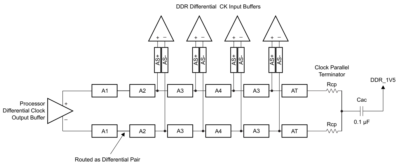
Figure 7-6. CK Topology for Four x8 DDR3 Devices
