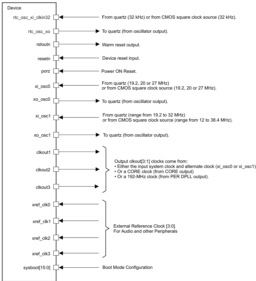
Figure 5-8. Clock Interface
