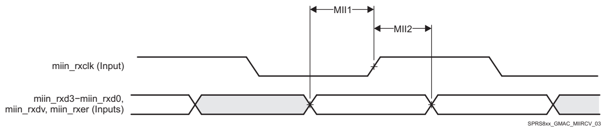
Figure 5-70. GMAC Receive Interface Timing MII operation
