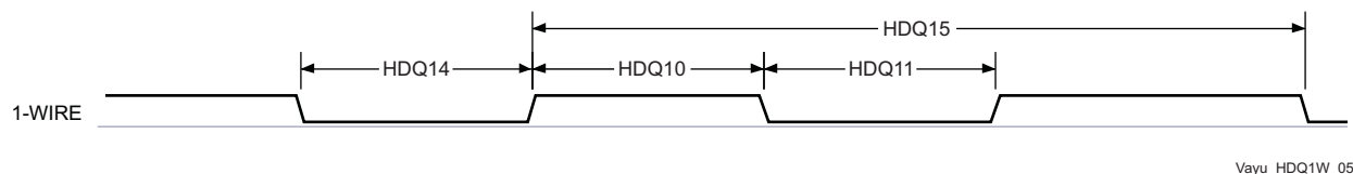
Figure 5-46. 1-Wire—Break (Reset)
