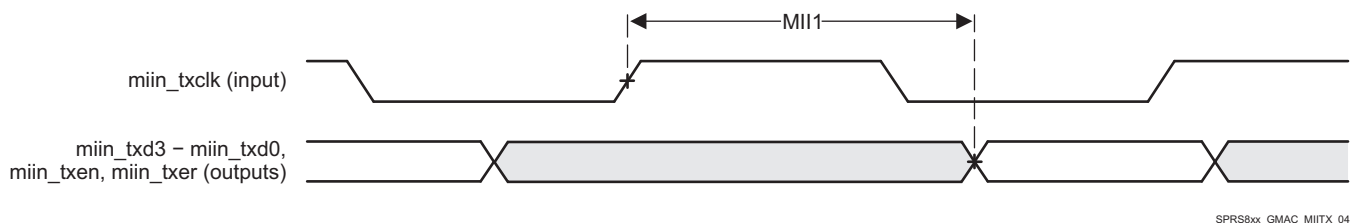
Figure 5-71. GMAC Transmit Interface Timing MII operation
