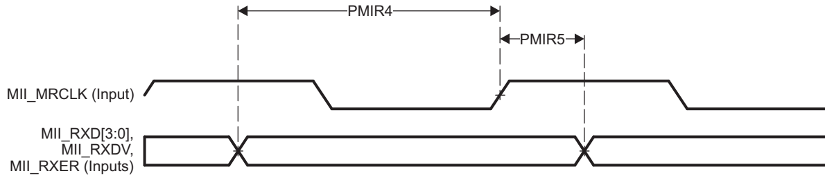
Figure 5-126. PRU-ICSS MII_RXD[3:0], MII_RXDV, and MII_RXER Timing
