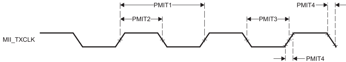
Figure 5-125. PRU-ICSS MII[x]_TXCLK Timing
