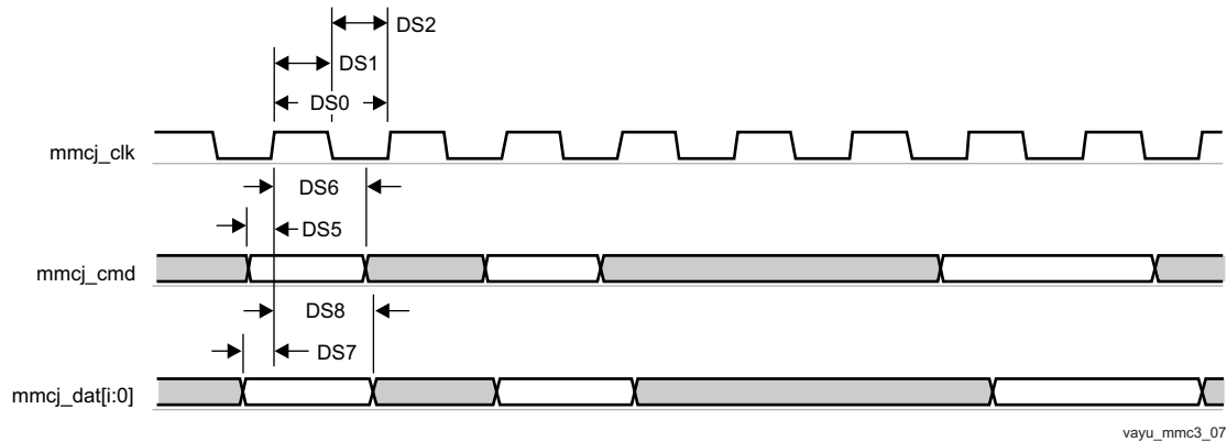
Figure 5-98. MMC/SD/SDIOj in - Default Speed - Receiver Mode
