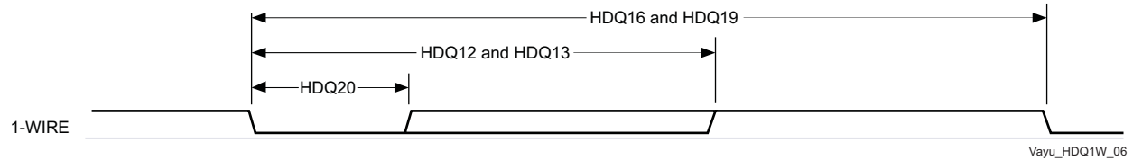
Figure 5-47. 1-Wire—Read Bit (Data)
