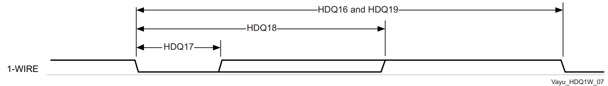
Figure 5-48. 1-Wire—Write Bit-One Timing (Command / Address or Data)
