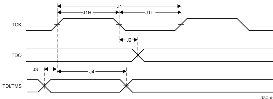
Figure 5-129. JTAG Timing
