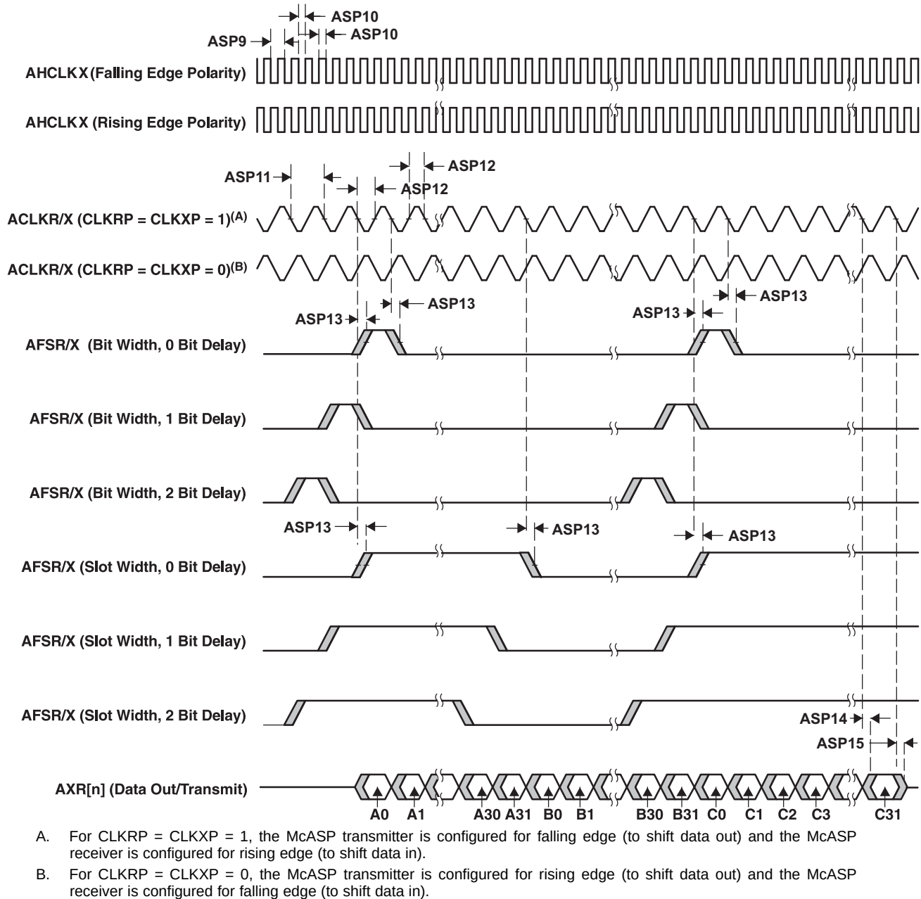
Figure 5-59. McASP Output Timing
