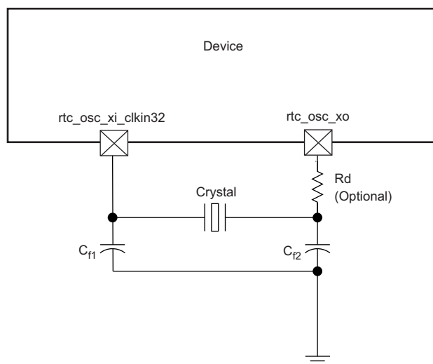
Figure 5-17. Crystal Implementation
