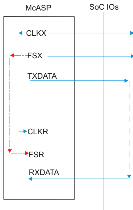
Figure 5-64. McASP1-8 CO-FO- – SYNC Mode
