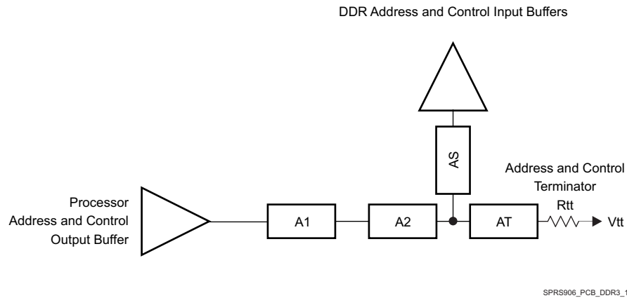
Figure 8-19. ADDR_CTRL Topology for One DDR3 Device
