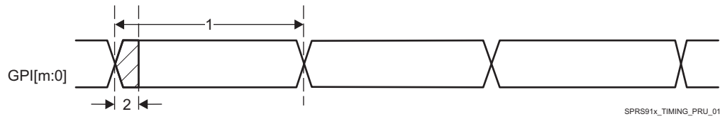
Figure 7-92. PRU-ICSS PRU Direct Input Timing
