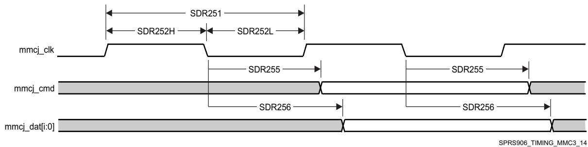
Figure 7-89. MMC/SD/SDIOj in - SDR25 - Transmitter Mode
