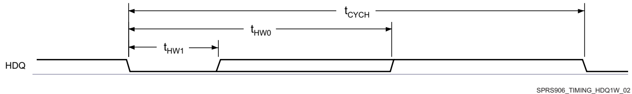
Figure 7-26. Device HDQ Interface Bit Read Timing (Data)
