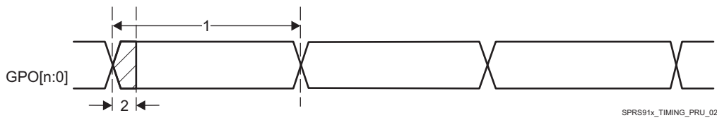
Figure 7-93. PRU-ICSS PRU Direct Output Timing
