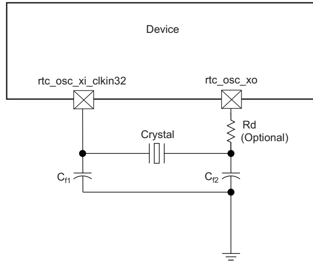
Figure 8-32. Grounding Scheme for Low-Frequency Clock
