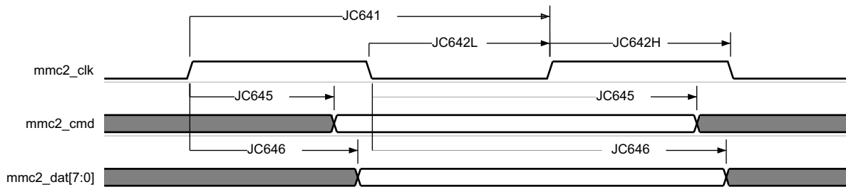
Figure 7-78. MMC/SD/SDIO in - High Speed JC64 - Transmitter Mode
