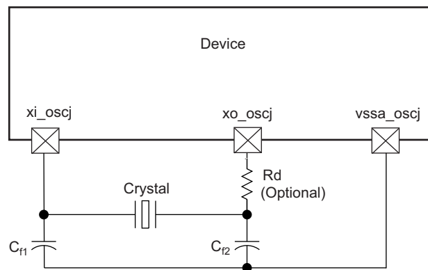
Figure 8-33. Grounding Scheme for High-Frequency Clock
