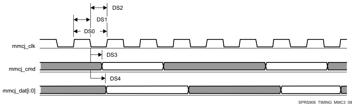
Figure 7-83. MMC/SD/SDIOj in - Default Speed - Transmitter Mode
