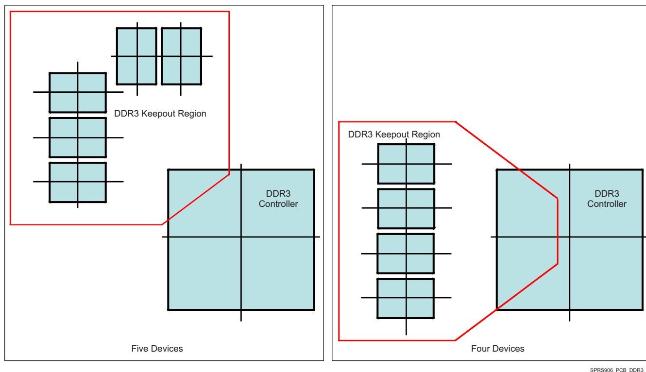
Figure 8-5. DDR3 Keepout Region
