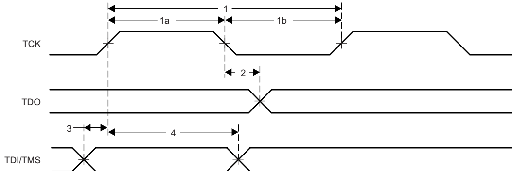
Figure 7-113. JTAG Timing
