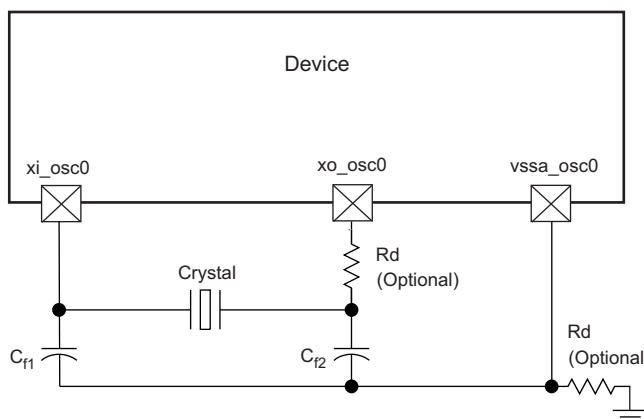
Figure 6-2. Crystal Implementation
