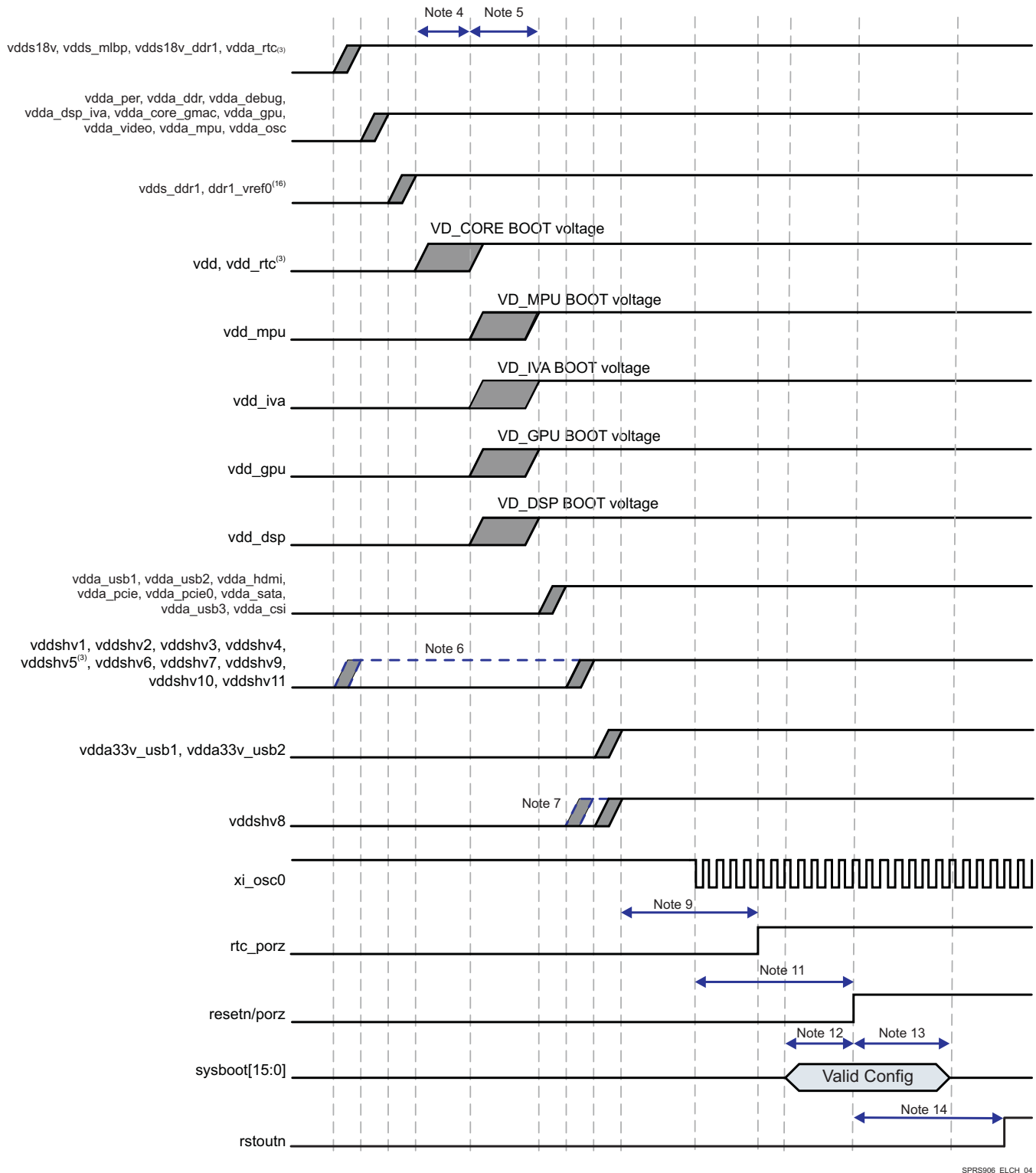
Figure 5-2. Power-Up Sequencing
