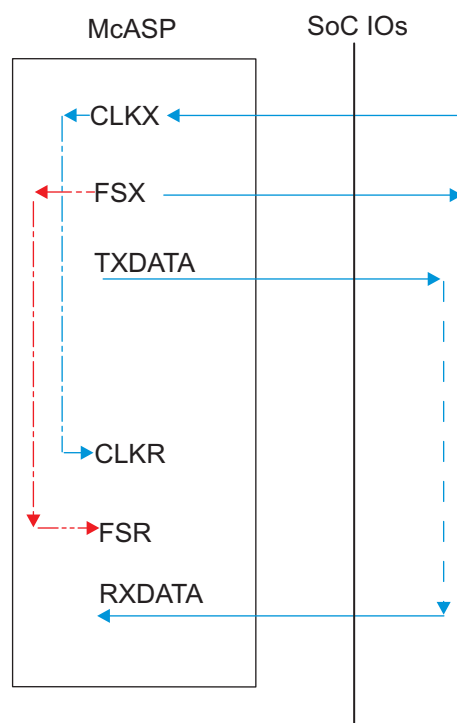
Figure 7-48. McASP1-8 CI-FO - SYNC Mode
