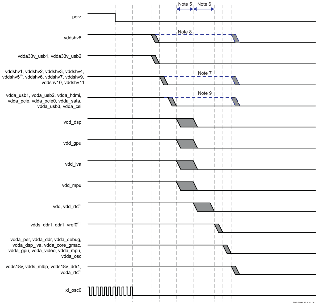
Figure 5-3. Power-Down Sequencing (10)(12)
