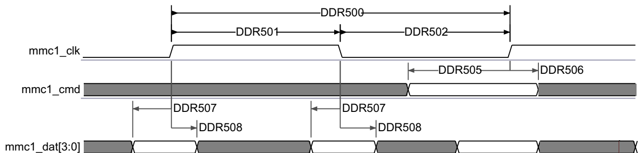
Figure 5-85. SDMMC - High Speed SD - DDR - Data/Command Receive
