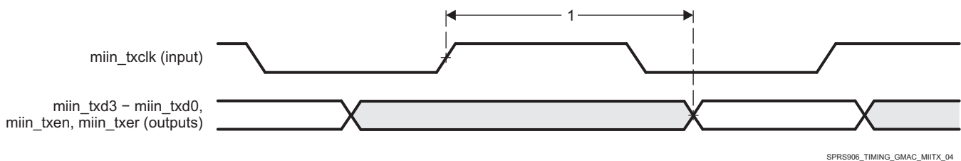
Figure 5-67. GMAC Transmit Interface Timing MIIn operation
