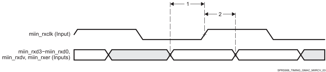
Figure 5-66. GMAC Receive Interface Timing MIIn operation
