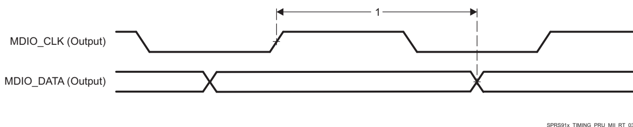
Figure 5-119. PRU-ICSS MDIO_DATA Timing – Output Mode
