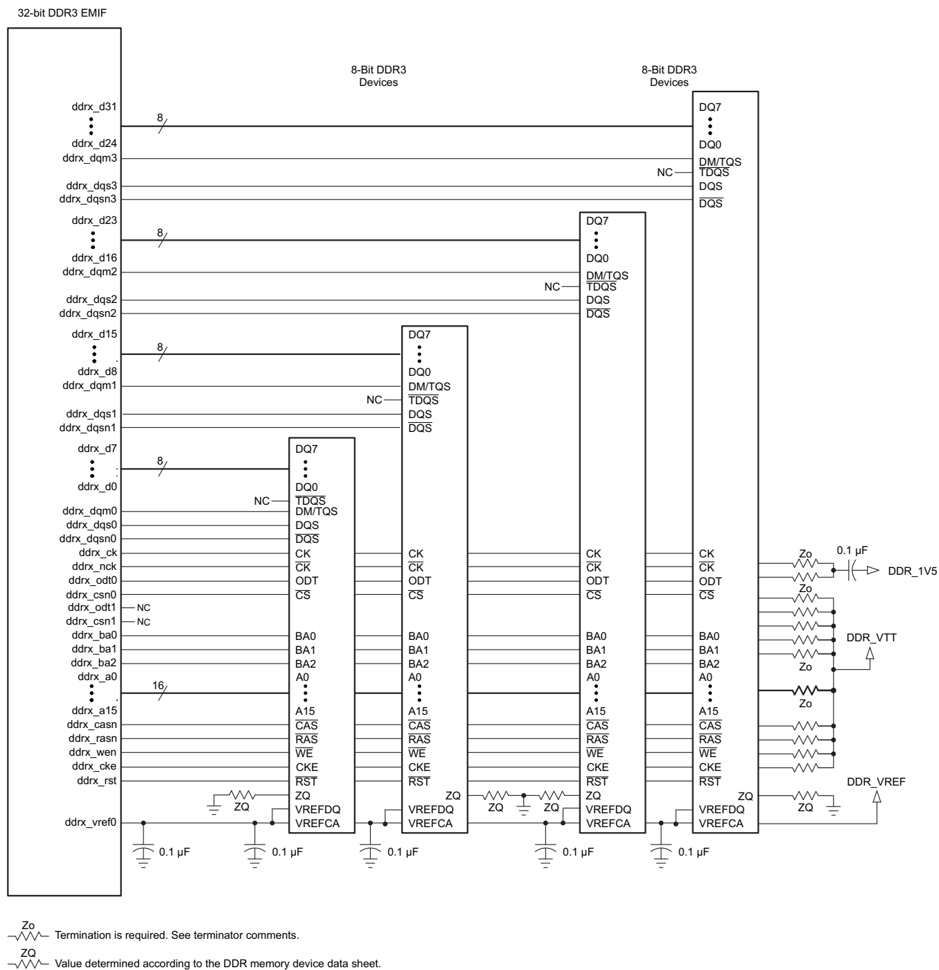
Figure 7-3. 32-Bit, One-Bank DDR3 Interface Schematic Using Four 8-Bit DDR3 Devices
