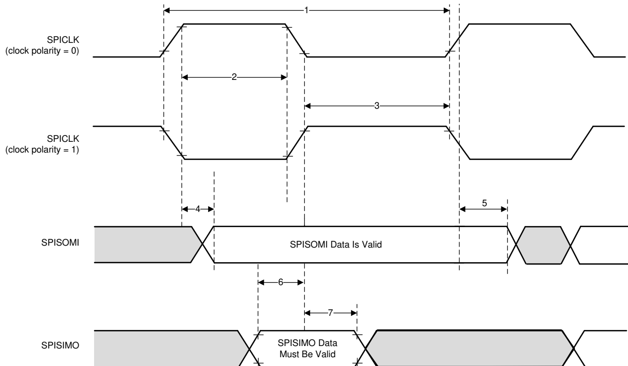
Figure 6-9. SPI Slave Mode External Timing (CLOCK PHASE = 0)
