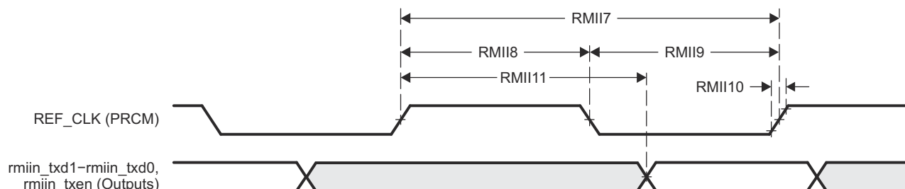
Figure 6-13. GMAC Transmit Interface Timing RMII In Operation
