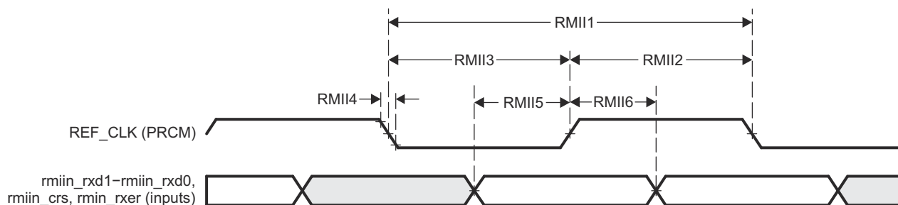
Figure 6-14. GMAC Receive Interface Timing RMII In operation
