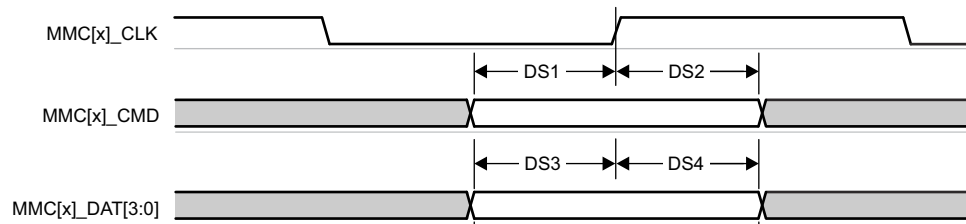
Figure 6-28. MMC – Default Speed – Receive Mode
