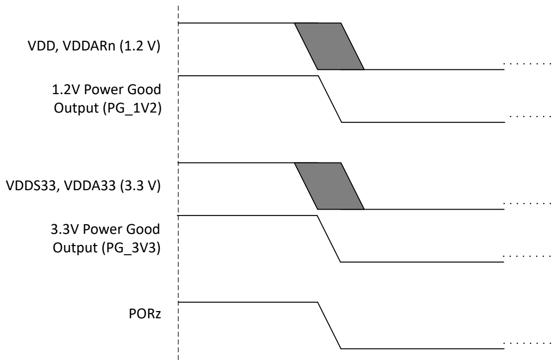
Figure 6-3. Power-Down Sequencing
