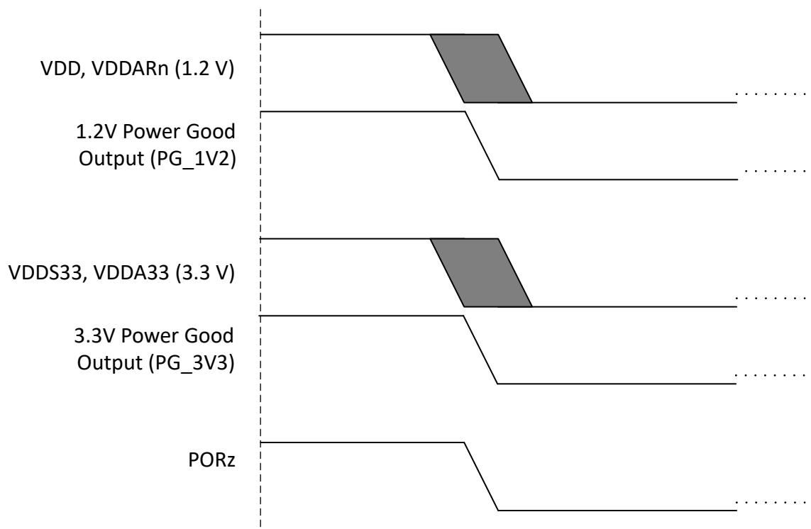
Figure 7-2. Power-Down Sequencing
