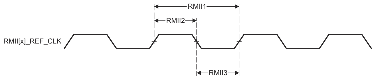
Figure 6-13. CPSW RMII[x]_REF_CLK Timing Requirements – RMII Mode
