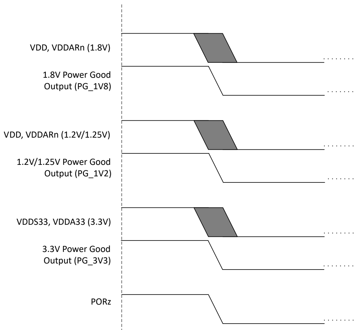
Figure 6-3. Power-Down Sequencing
