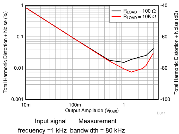
Figure 6-10. THD+N vs Output Amplitude
