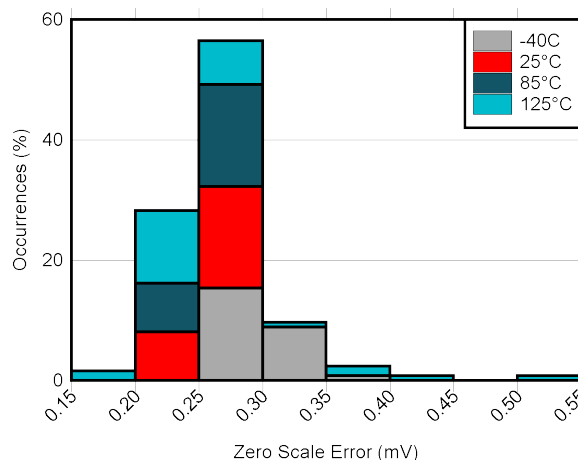
Figure 5-18. DAC Zero Scale Error vs Temperature
