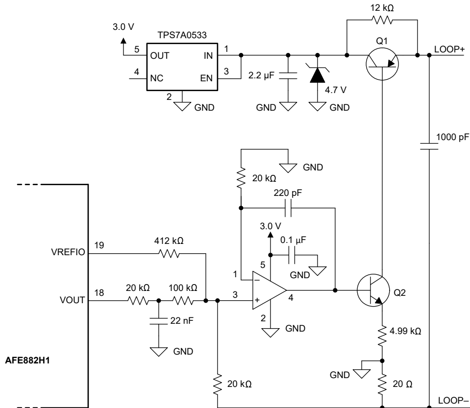
Figure 8-4. Current Loop Control for the AFE882H1 Transmitter
