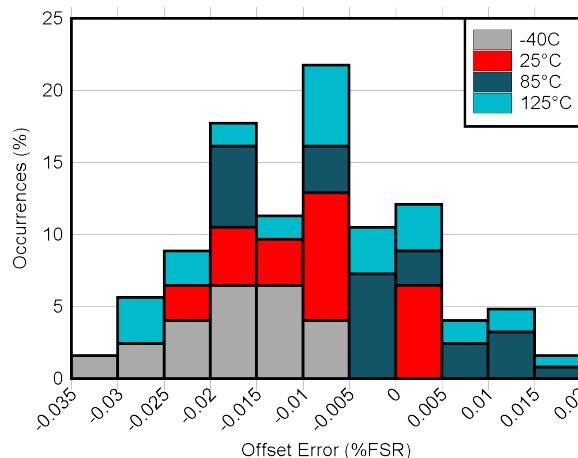
Figure 5-16. DAC Offset Error vs Temperature
