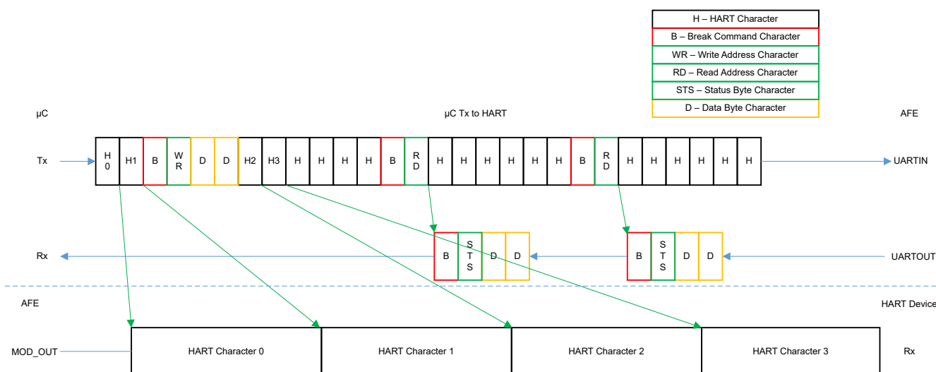
Figure 6-37. Packed HART Transmit With UBM Register Write and Read Requests and Responses
