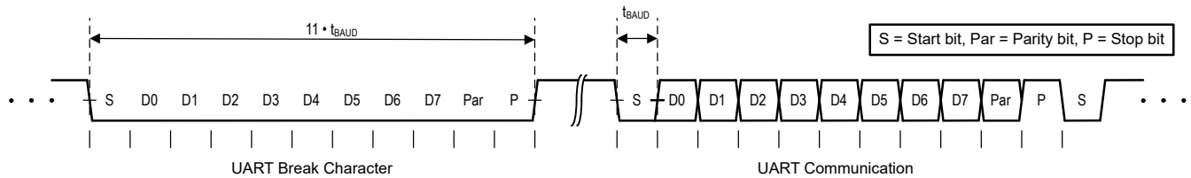
Figure 5-2. UBM Timing
