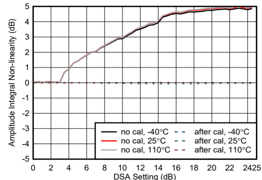
Figure 4-451. RX Amplitude Integrated Non-linearity at 9.6 GHz
