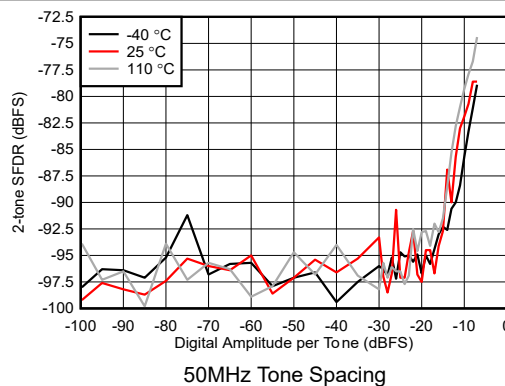
Figure 4-429. RX 2-tone SFDR vs Digital Amplitude at 8.11 GHz
