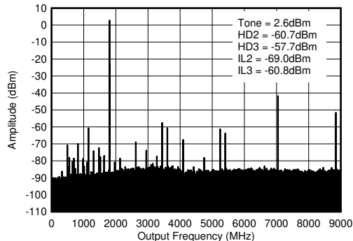
Figure 4-73. TX Single Tone (-12 dBFS) Output Spectrum at 1.8 GHz ( 0-f_{\text{DAC}} )
