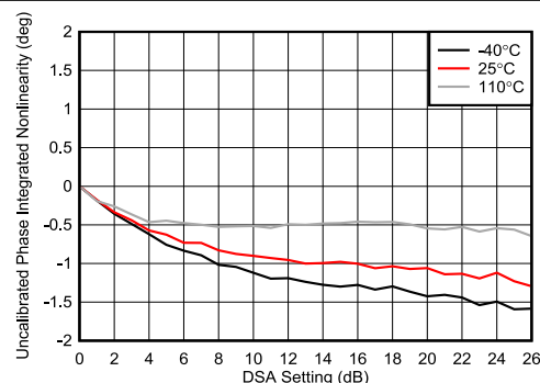
Figure 4-244. TX DSA Uncalibrated Phase Integrated Nonlinearity
