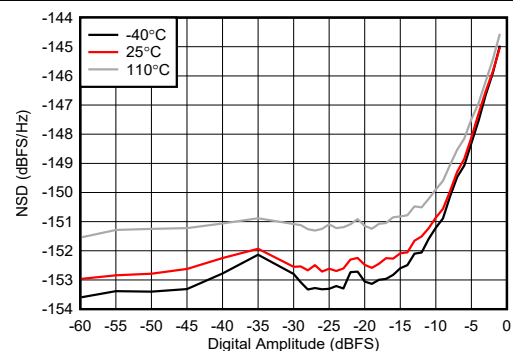
Figure 4-254. TX NSD vs Digital Amplitude at 9.61 GHz
