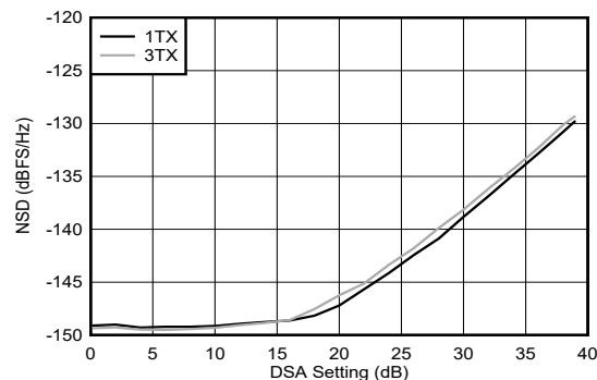
Figure 4-256. TX NSD vs DSA Setting at 9.61 GHz
