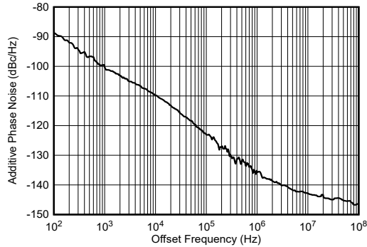
Figure 4-269. TX Additive Phase Noise vs Offset Frequency at 9.61 GHz
