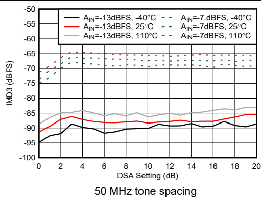
Figure 4-419. RX IMD3 vs DSA Setting at 8.11 GHz
