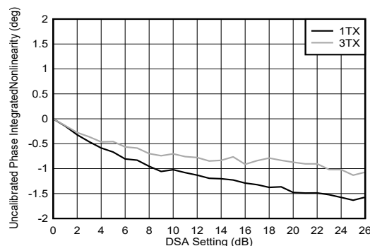
Figure 4-242. TX DSA Uncalibrated Phase Integrated Nonlinearity
