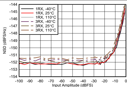
Figure 4-421. RX NSD vs Digital Amplitude at 8.11 GHz
