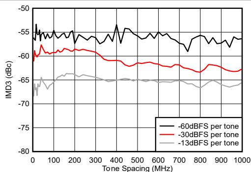
Figure 4-251. TX IMD3 vs Tone Spacing at 9.61 GHz
