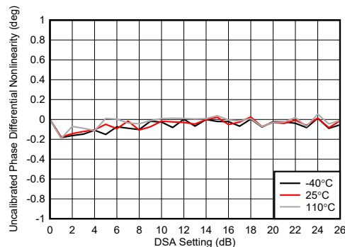
Figure 4-240. TX DSA Uncalibrated Phase Differential Nonlinearity
