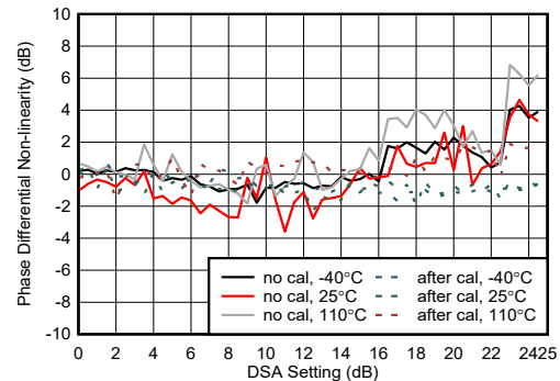
Figure 5-449. RX Phase Integrated Non-linearity at 9.6 GHz
