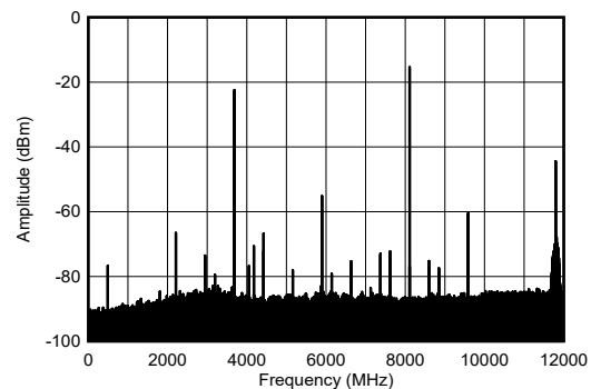
Figure 4-205. TX Single Tone Output Spectrum at 8.11GHz
