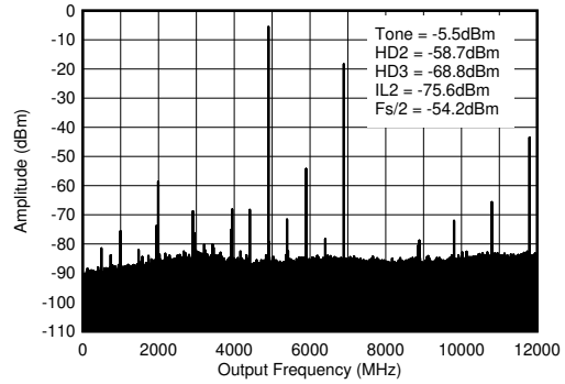
f_{\text{DAC}} = 11796.48\text{MSPS} , interleave mode, 4.9GHz matching, includes PCB and cable losses. \text{ILn} = f_{\text{S}}/\text{n} \pm f_{\text{OUT}} .
