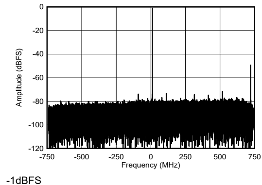
Figure 4-466. RX Single Tone Output FFT at 9.61 GHz
