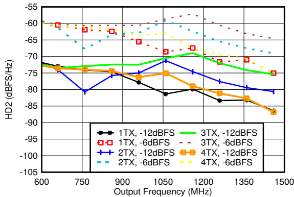
Matching at 0.8GHz, f_{DAC} = 5898.2\text{GSPS} , straight mode
