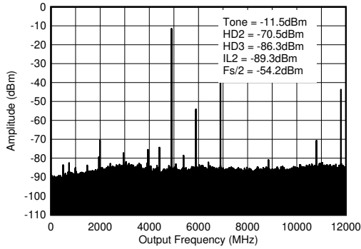
f_{\text{DAC}} = 11796.48\text{MSPS} , interleave mode, 4.9GHz matching, includes PCB and cable losses. \text{ILn} = f_{\text{S}}/\text{n} \pm f_{\text{OUT}} .
