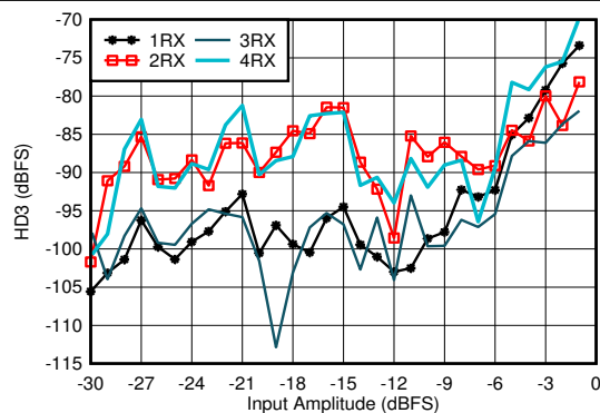
Figure 5-75. RX HD3 vs Input Level and Channel at 0.8 GHz
