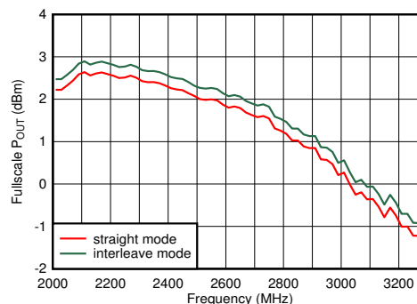
Figure 5-354. TX Full Scale vs RF Frequency at 8847.36MSPS
