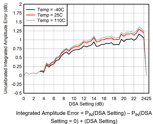
Figure 5-32. RX Uncalibrated Integrated Amplitude Error vs DSA Setting at 400 MHz
