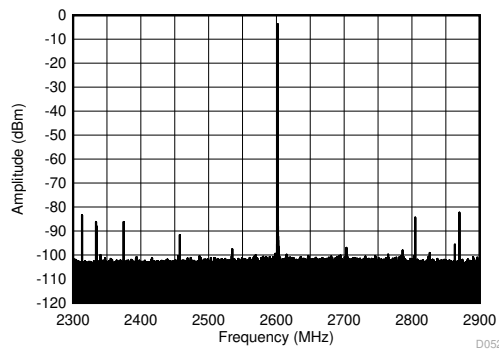
Figure 5-396. TX Single Tone (-12 dBFS) Output Spectrum at 2.6 GHz ( \pm 300\text{ MHz} )
