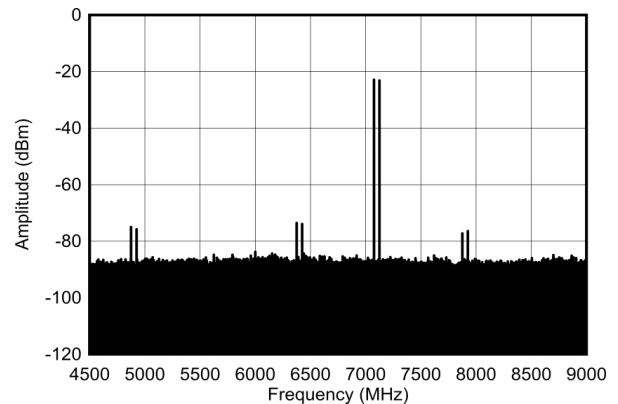
Figure 5-561. Two Tone Output Spectrum at 7.1GHz, -7dBFS each (Nyquist)
