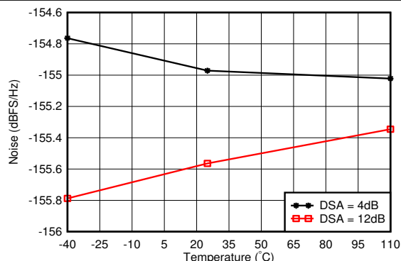
Figure 5-93. RX Noise Spectral Density vs Temperature at 1.75 GHz
