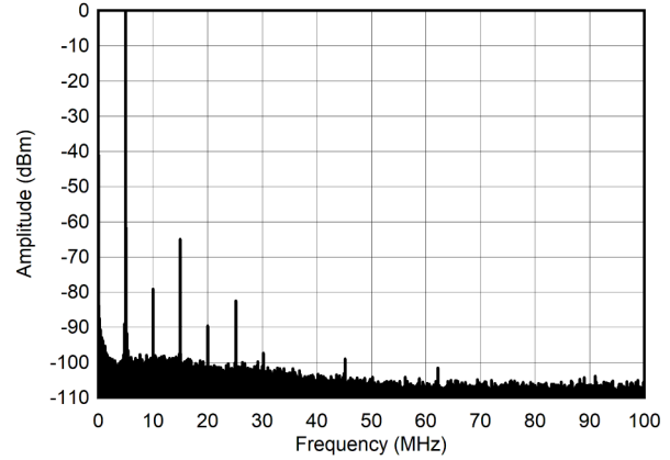
Figure 5-215. Single Tone Spectrum at 5 MHz and -6d BFS (0 - 100 MHz)
