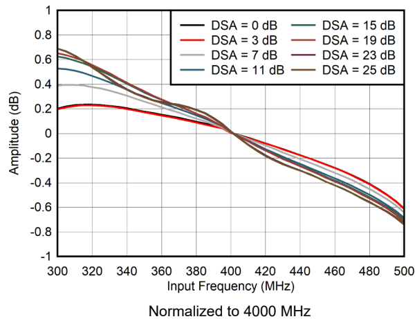
Figure 5-29. RX In-Band Gain Flatness, f_{\text{IN}} = 400 MHz
