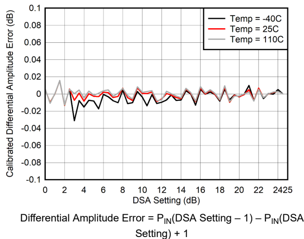
Figure 5-31. RX Calibrated Differential Amplitude Error vs DSA Setting at 400 MHz
