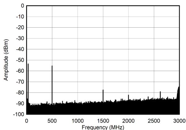
Figure 5-227. Single Tone Spectrum at 30 MHz and -60 dBFS (Nyquist)
