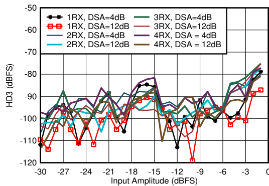
Figure 5-105. RX HD3 vs Input Level and Channel at 1.9 GHz
