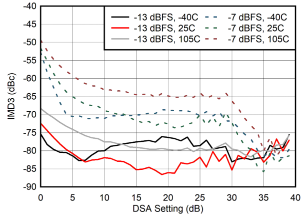
Figure 5-269. IMD3 vs DSA Setting at 400 MHz
