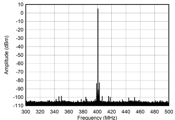
Figure 5-249. Single Tone Spectrum at 400 MHz and -1 dBFS ( \pm 100\text{MHz} )
