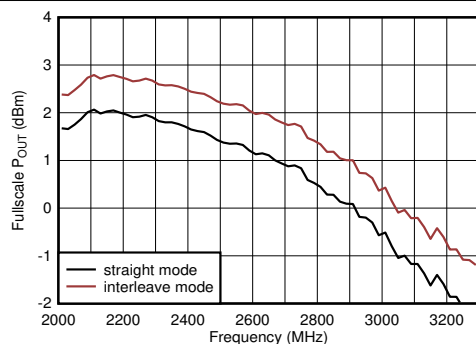
Figure 5-353. TX Full Scale vs RF Frequency at 5898.24MSPS
