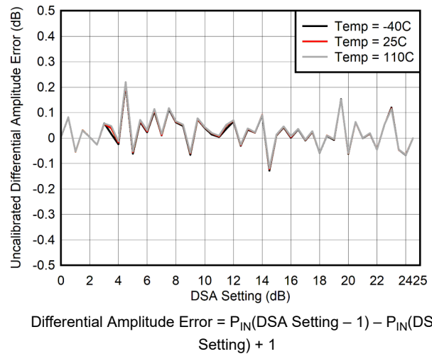
Figure 5-30. RX Uncalibrated Differential Amplitude Error vs DSA Setting at 30 MHz
