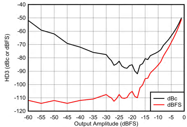
Figure 5-271. HD3 vs Amplitude at 400 MHz
