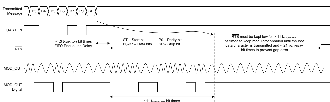
Figure 7-22. HART Transmit End Timing Diagram (UBM, UART Plus SPI Modes)
