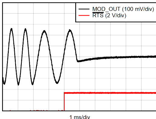
Figure 8-9. \overline{\text{RTS}} Stop Timing
