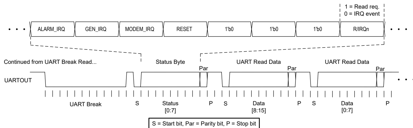
Figure 7-33. UARTOUT Break Data Format
