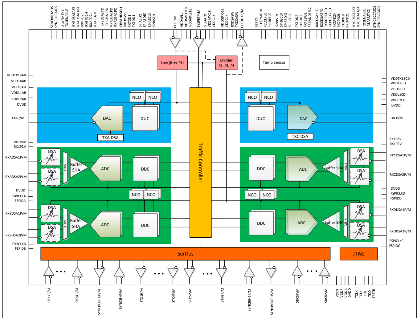
Figure 1-2. Functional Block Diagram of AFE7684
