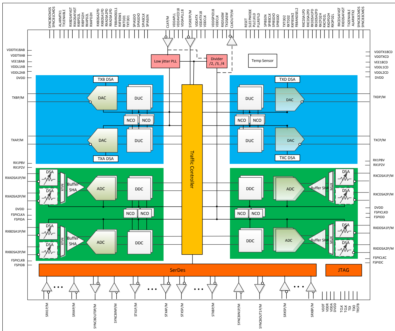
Figure 1-1. Functional Block Diagram of AFE7685/AFE7686
