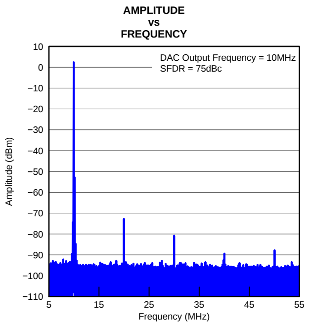
Figure 6-18. Spectrum Analyzer Plot CMOS Mode 10MHz IF
