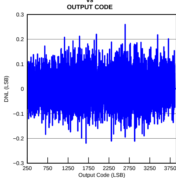
Figure 6-16. DNL Plot
