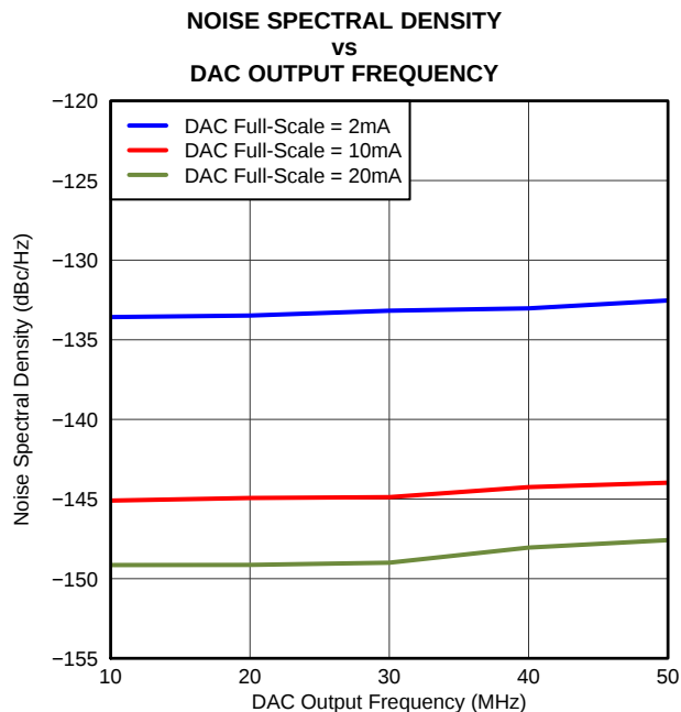
Figure 6-21. NSD Vs louts
