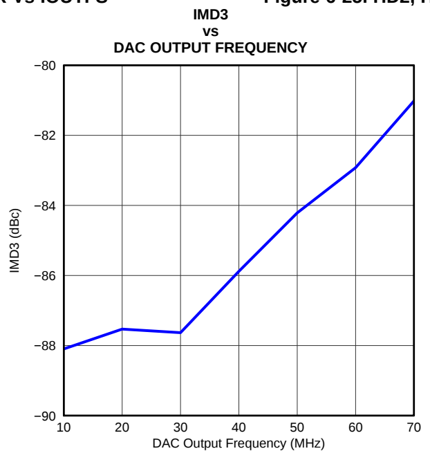
Figure 6-26. IMD3 vs Frequency CMOS
