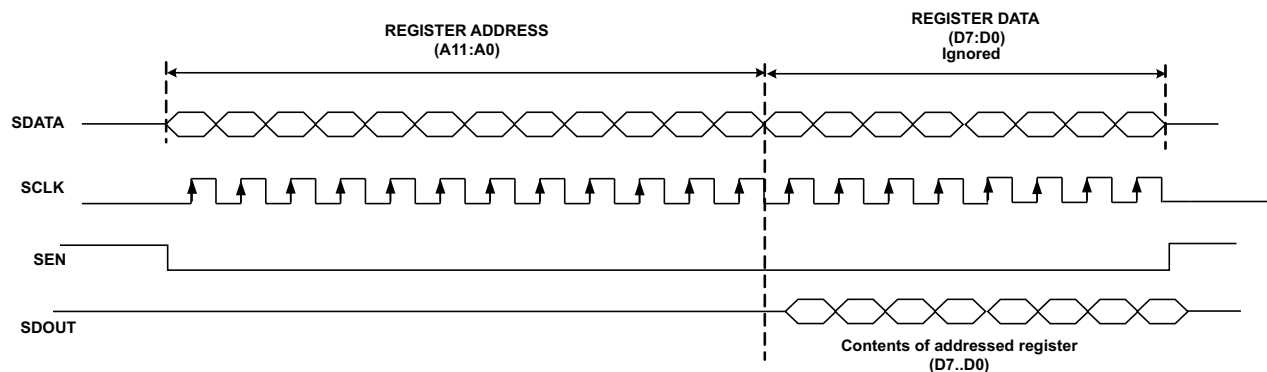
Figure 4-2. Timing
