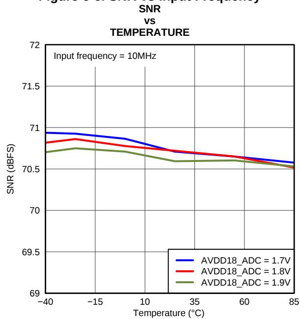
Figure 6-8. SNR Across Temperature and ADC Analog Supply
