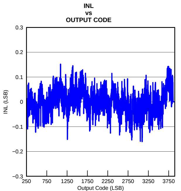
Figure 6-17. INL Plot
