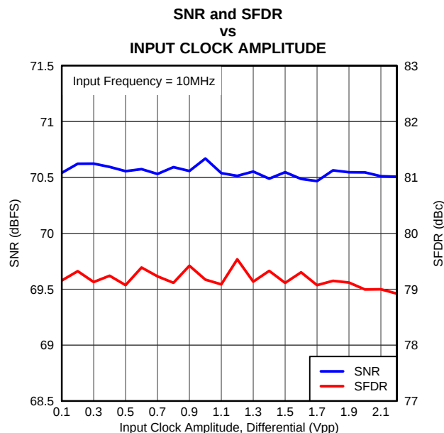
Figure 6-13. Performance Across Input Clock Amplitude
