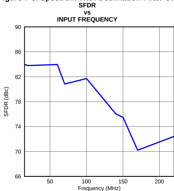
Figure 7-7. SFDR vs Input Frequency
