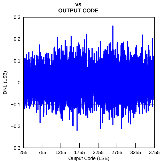
Figure 7-16. DNL Plot
