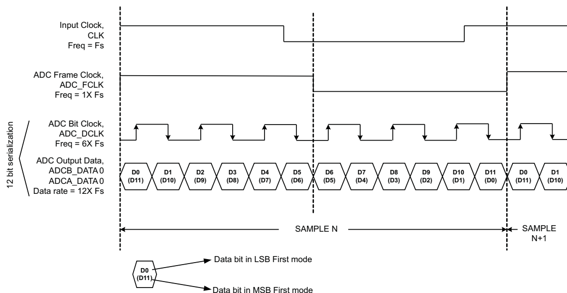
Figure 10-11. 1-WIRE MODE
