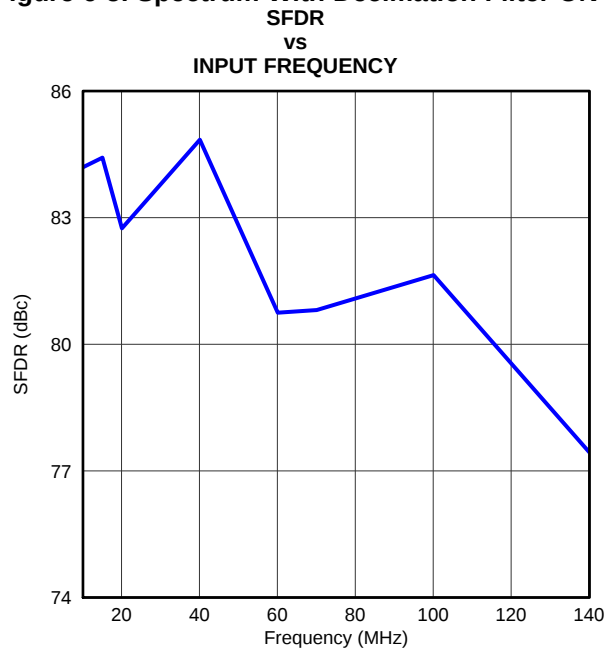
Figure 6-7. SFDR vs Input Frequency
