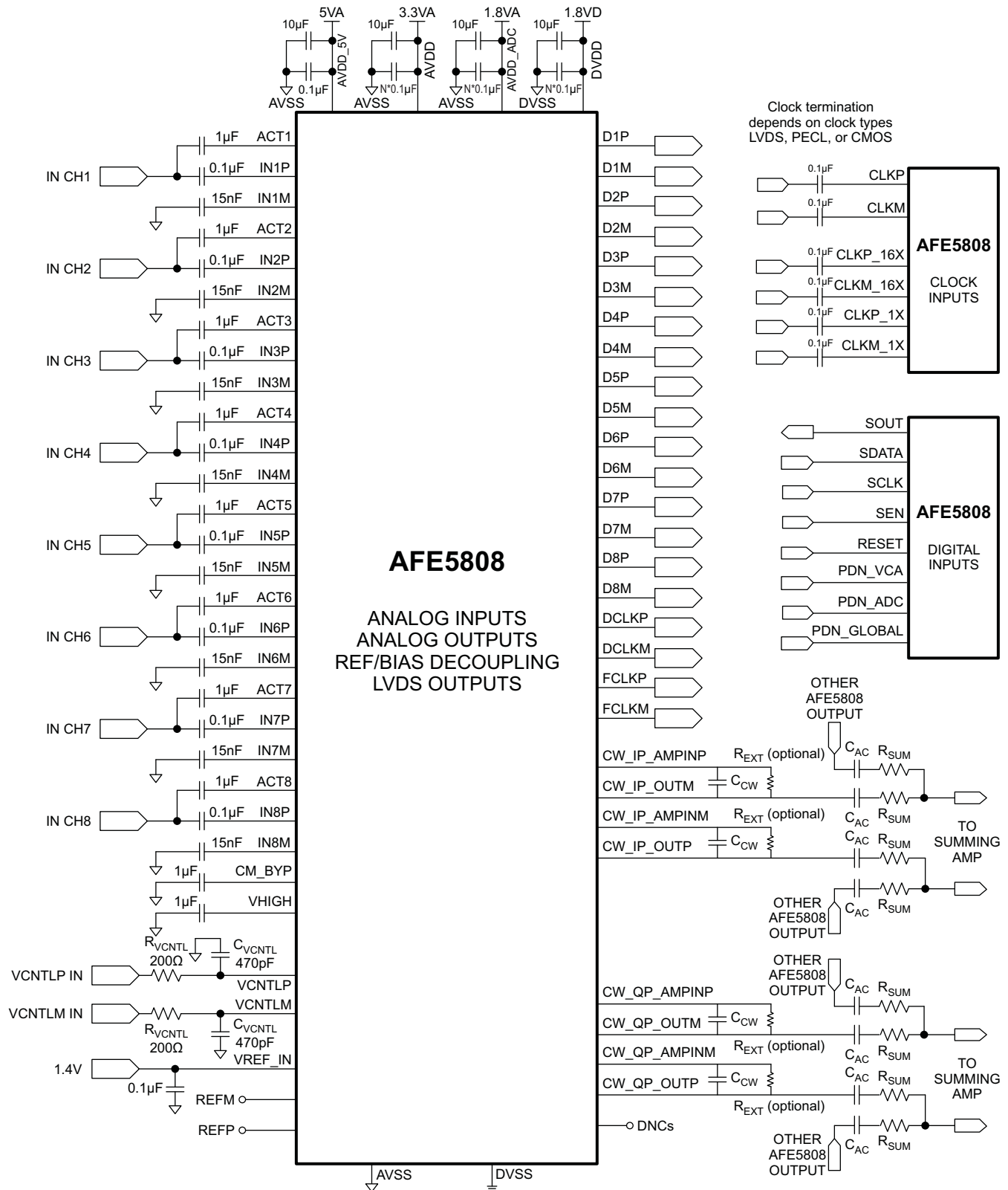
Figure 81. Application Circuit
