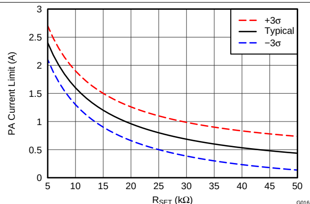
Figure 20. PA Current Limit vs R_{SET}
