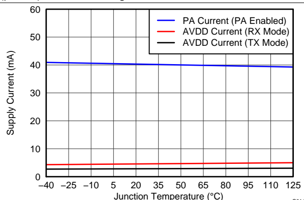
Figure 14. Quiescent Supply Current vs Temperature
