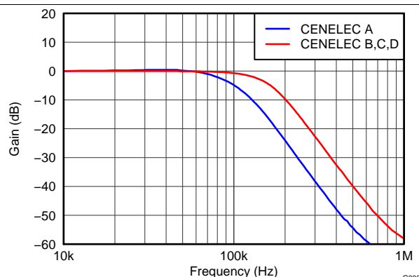
Figure 2. Rx Filter Gain vs Frequency
