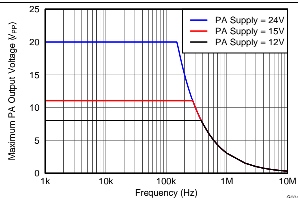
Figure 4. Maximum PA Output Voltage vs Frequency
