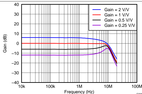
Figure 6. Rx PGA1 Gain vs Frequency
