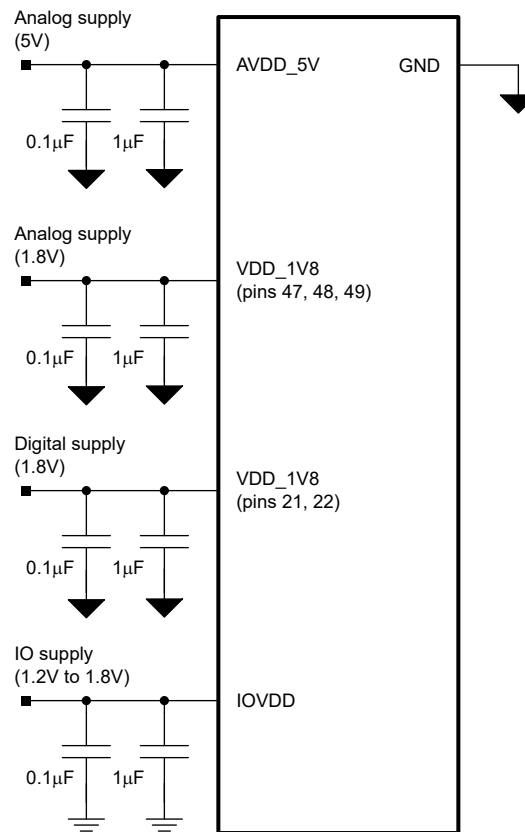
Figure 8-4. Power-Supply Decoupling
