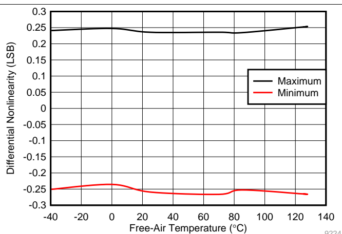
Figure 16. Typical DNL
