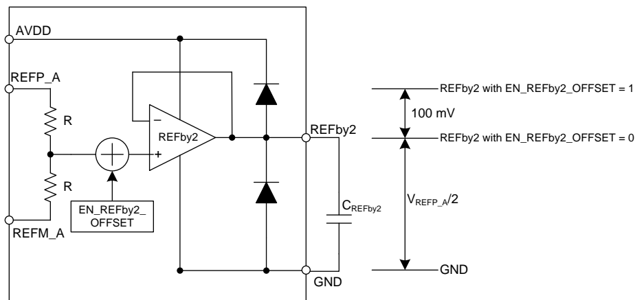
Figure 40. REFby2 Buffer
