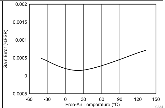
Figure 30. Gain Error vs Temperature
