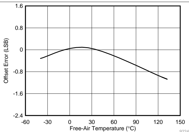
Figure 13. Offset Error vs Temperature
