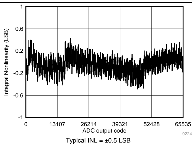
Figure 17. Typical INL
