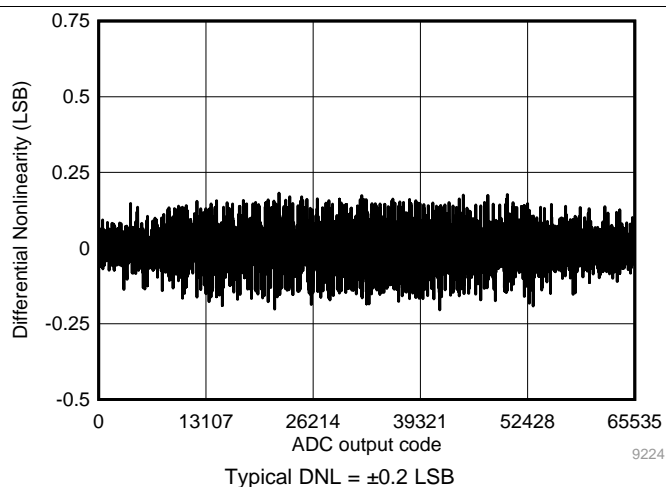
Figure 16. Typical DNL
