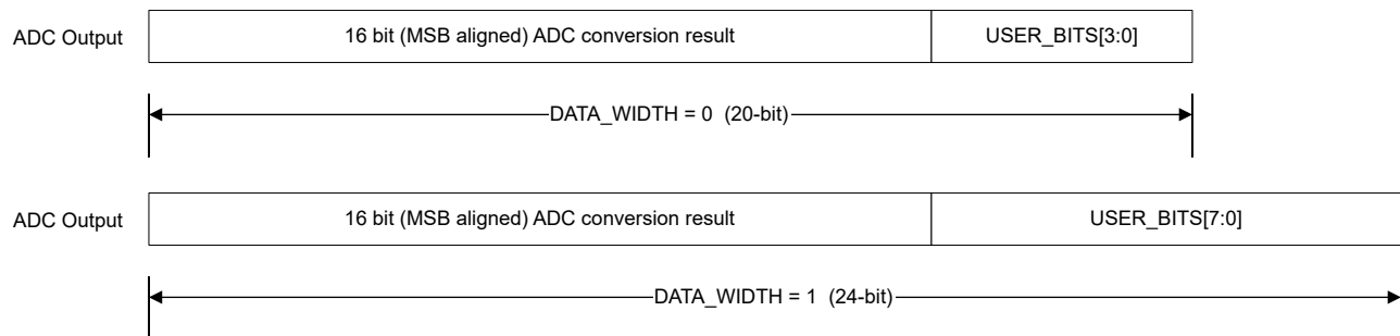
Figure 6-6. Data Frame Width Composition
