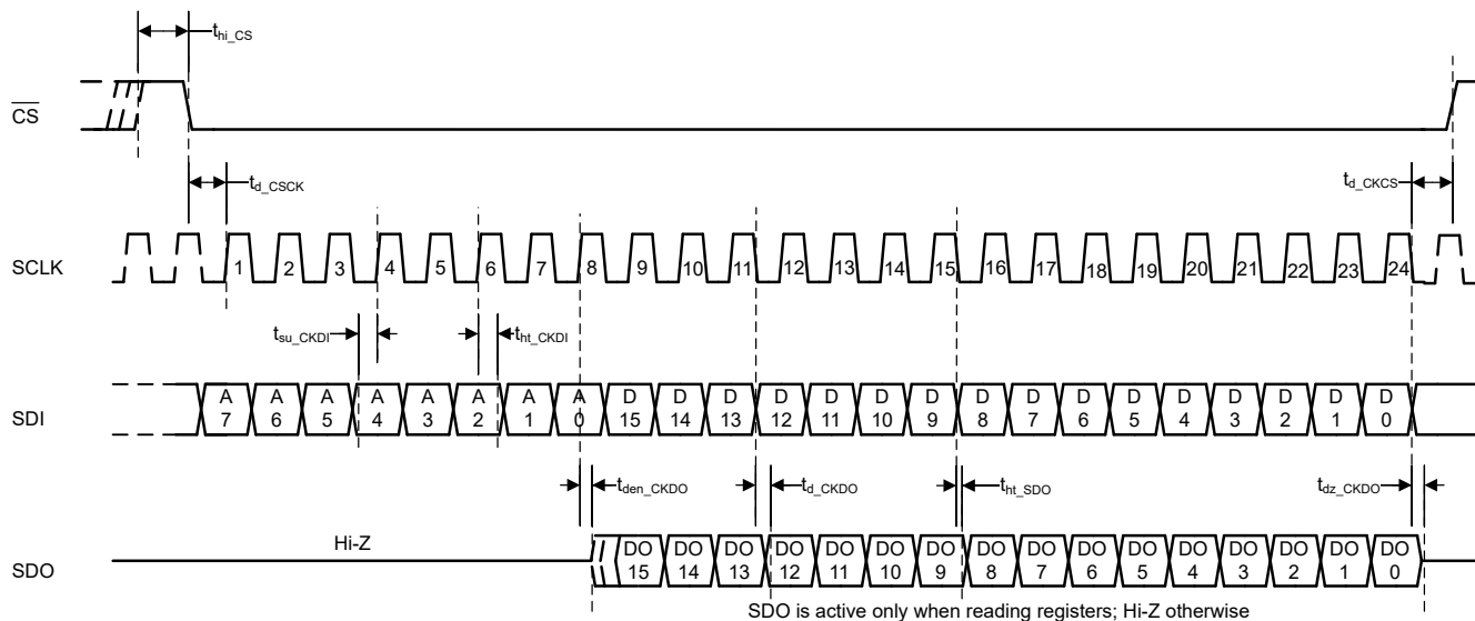
Figure 5-4. Configuration SPI
