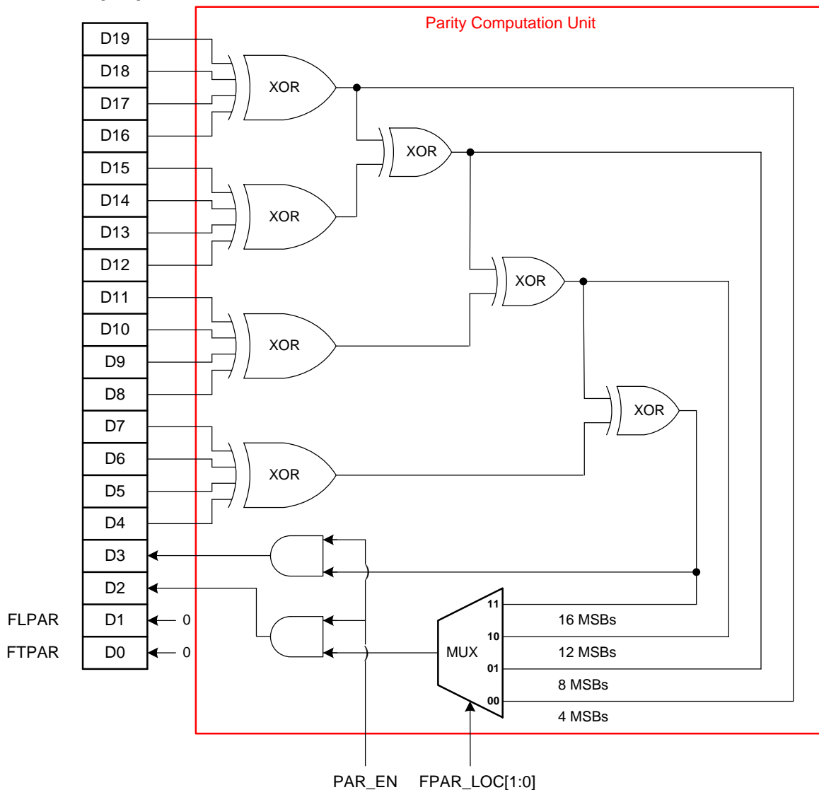
Figure 45. Parity Bits Computation
