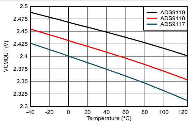
Figure 6-14. VCMOUT Voltage vs Temperature
