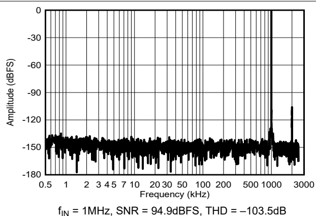
Figure 6-32. Typical FFT for f_{IN} = 1\text{MHz}
