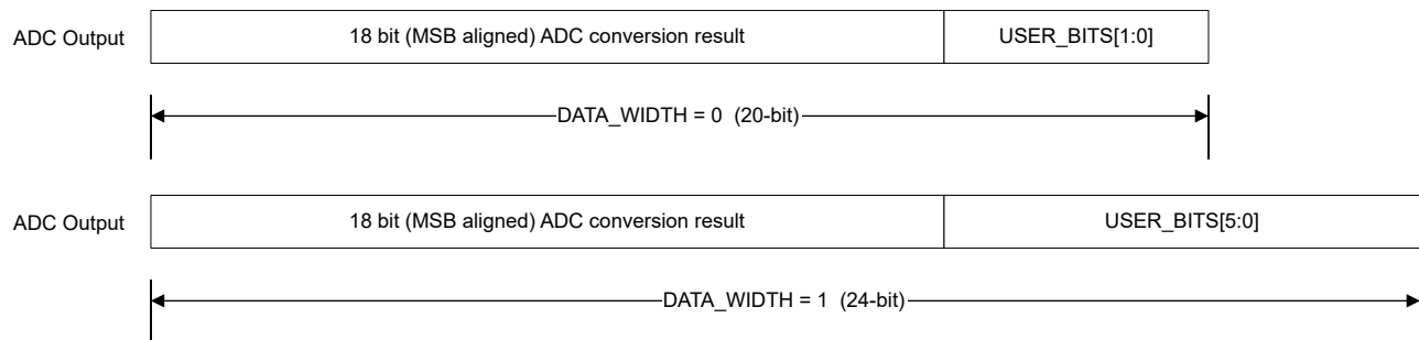
Figure 7-6. Data Frame Width Composition
