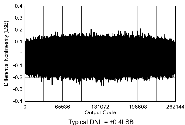
Figure 6-23. Typical DNL
