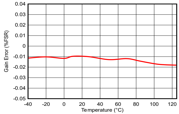
Figure 6-8. Gain Error vs Temperature
