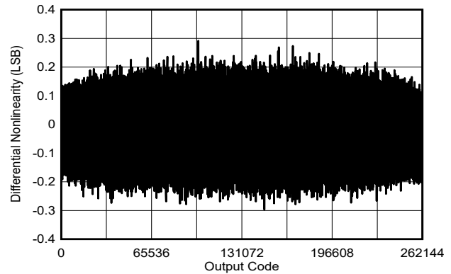
Typical DNL = \pm 0.4\text{LSB} Figure 6-18. Typical DNL
