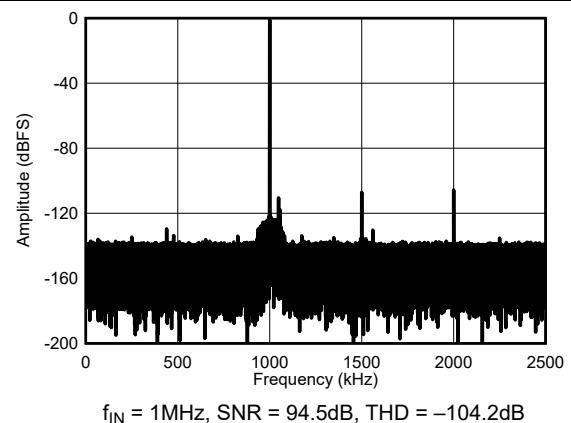
Figure 9-9. Typical FFT at 5MSPS/Channel: ADS9117
