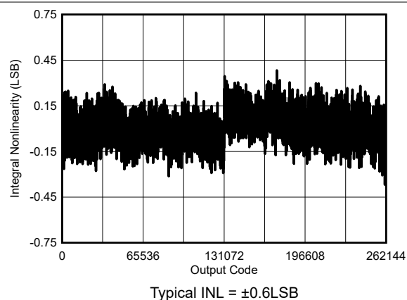
Figure 6-22. Typical INL
