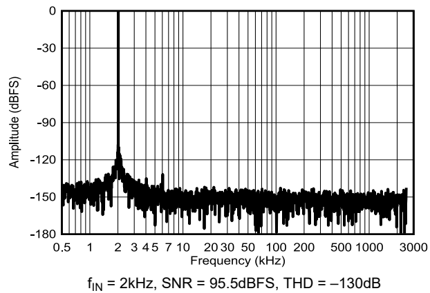
Figure 6-30. Typical FFT for f_{IN} = 2\text{kHz}
