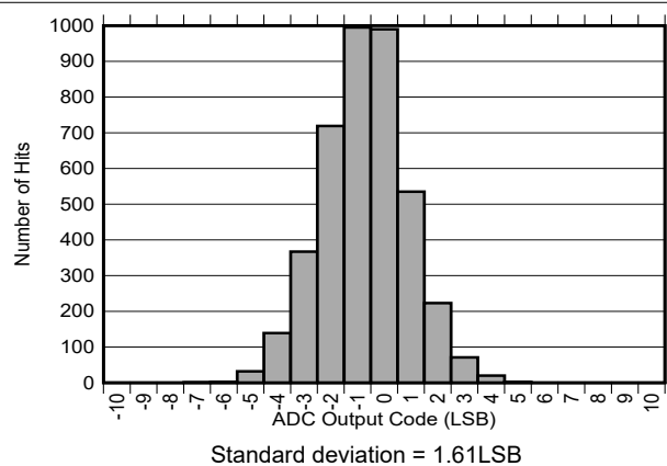
Figure 6-33. DC Input Histogram
