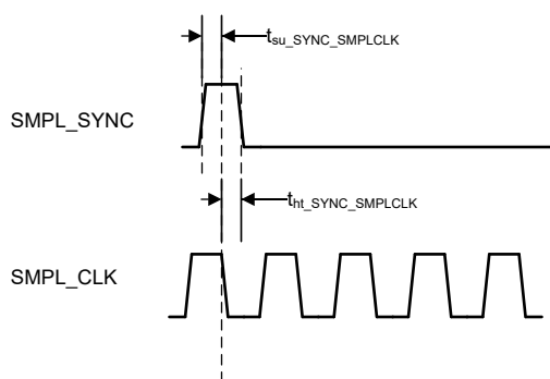
Figure 6-5. SMPL_SYNC Timing
