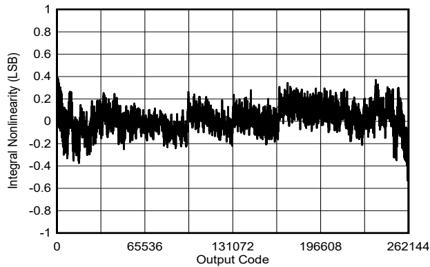
Typical INL = \pm 0.4\text{LSB} Figure 6-17. Typical INL
