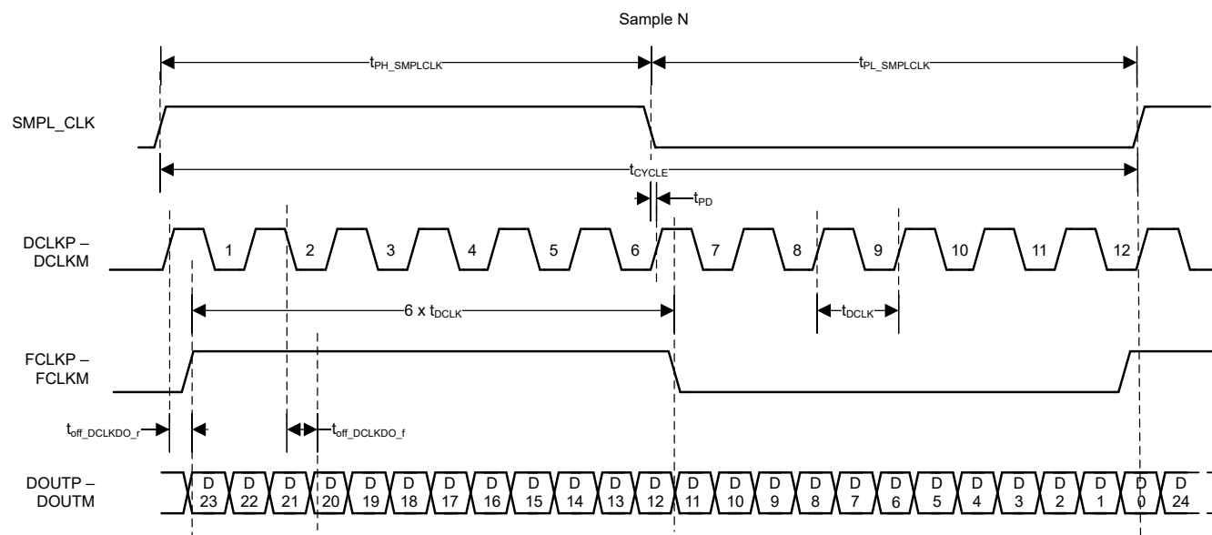
Figure 6-1. LVDS Data Interface: DDR
