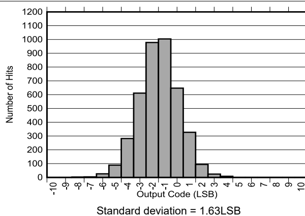
Figure 6-27. DC Input Histogram
