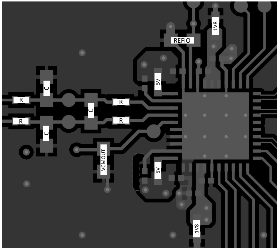
Figure 9-11. Example Layout
