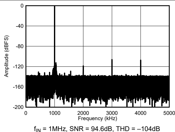
Figure 9-8. Typical FFT at 10MSPS/Channel: ADS9118
