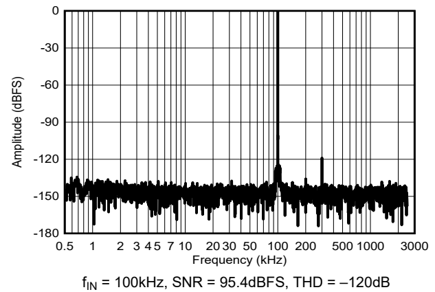
Figure 6-31. Typical FFT for f_{IN} = 100\text{kHz}
