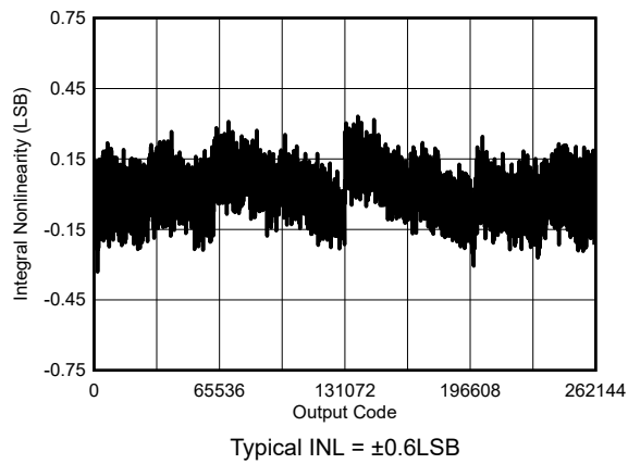
Figure 6-28. Typical INL
