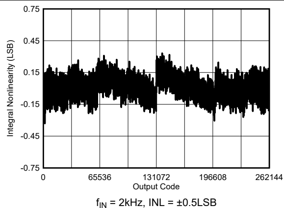
Figure 9-3. Typical INL at 5MSPS/Channel: ADS9117
