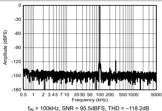
Figure 6-25. Typical FFT for f_{IN} = 100\text{kHz}
