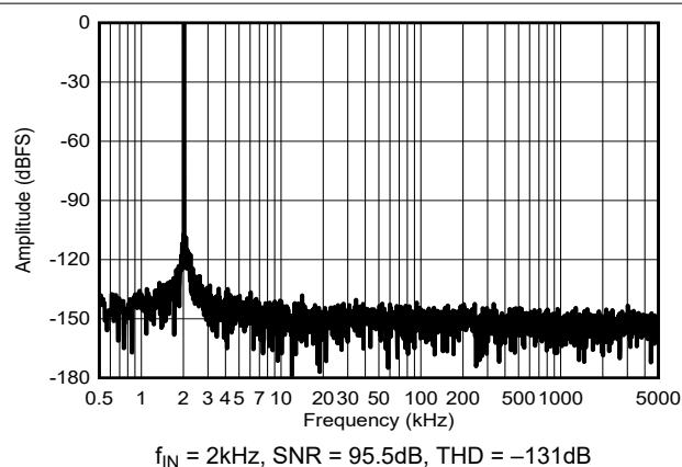
Figure 6-24. Typical FFT for f_{IN} = 2\text{kHz}
