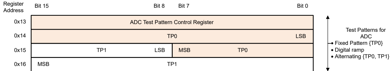
Figure 7-10. Register Bank for Test Patterns
