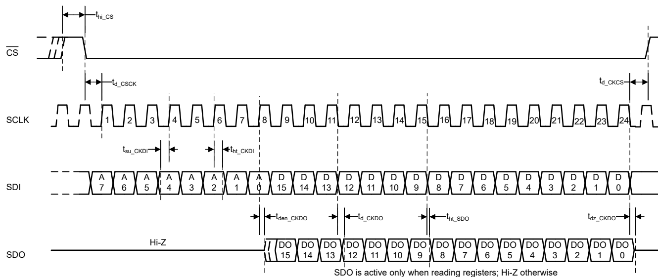
Figure 6-4. Configuration SPI
