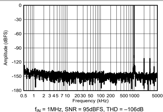
Figure 6-26. Typical FFT for f_{IN} = 1\text{MHz}
