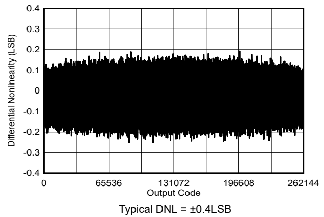
Figure 6-29. Typical DNL
