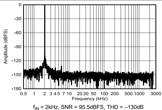
Figure 9-2. Typical FFT at 5MSPS/Channel: ADS9117
