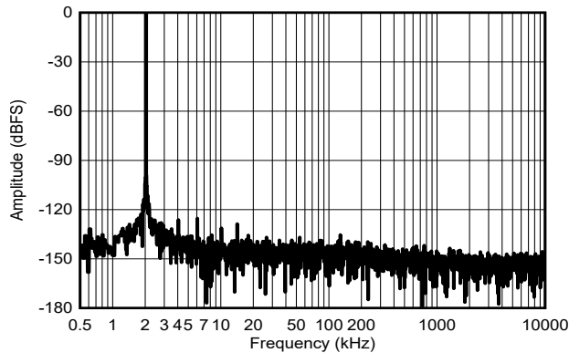
f_{IN} = 2\text{kHz} , SNR = 95.5dBFS, THD = -118\text{dB} Figure 6-19. Typical FFT for f_{IN} = 2\text{kHz}
