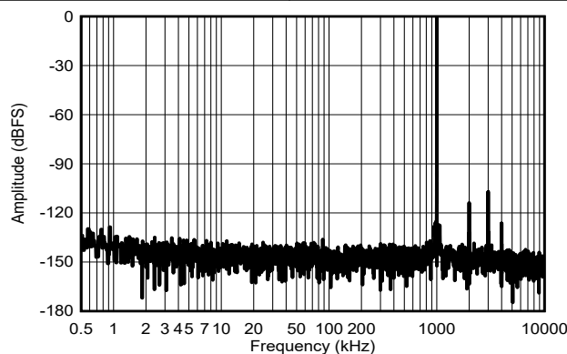
f_{IN} = 1\text{MHz} , SNR = 94.9dBFS, THD = -104.2\text{dB} Figure 6-21. Typical FFT for f_{IN} = 1\text{MHz}
