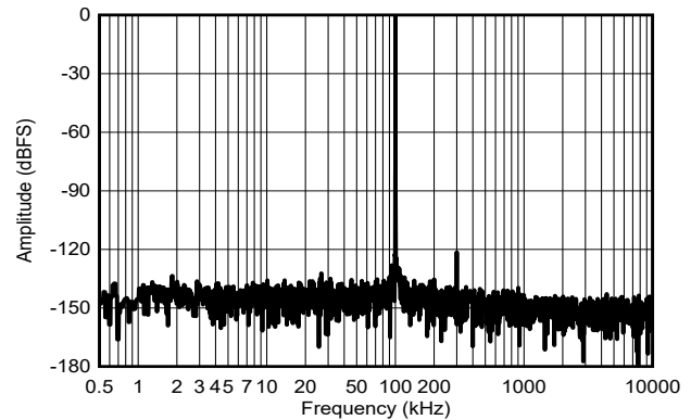
f_{IN} = 100\text{kHz} , SNR = 95.4dBFS, THD = -118\text{dB} Figure 6-20. Typical FFT for f_{IN} = 100\text{kHz}
