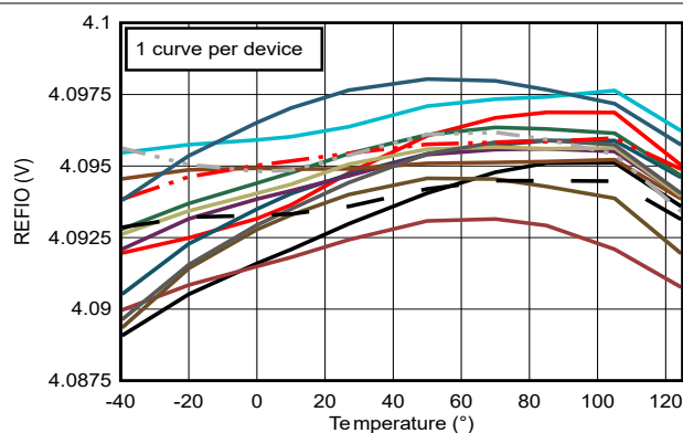
Figure 6-13. REFIO Voltage vs Temperature
