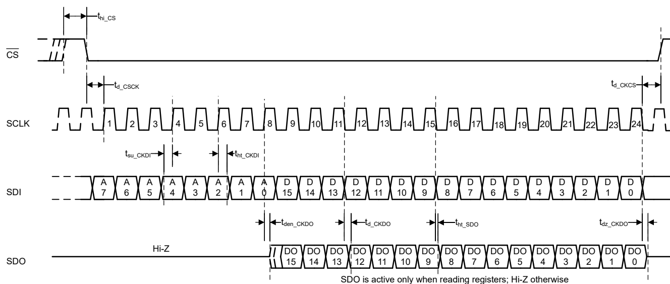
Figure 6-4. Configuration SPI
