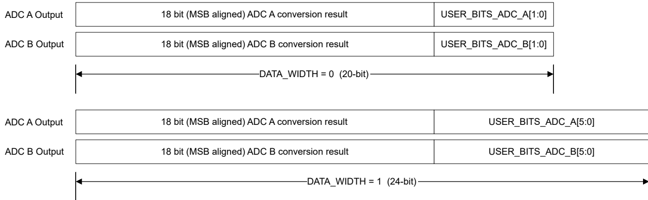
Figure 7-8. Data Frame Width Composition With LSB XOR Enabled
