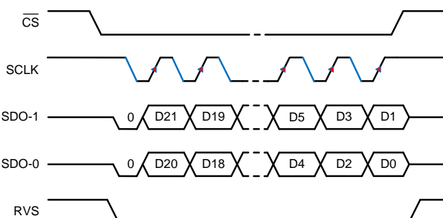
Figure 63. SPI-11-D Protocol
