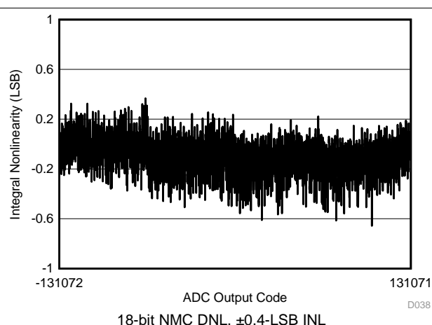
Figure 111. Typical Linearity, Single-Ended Input
