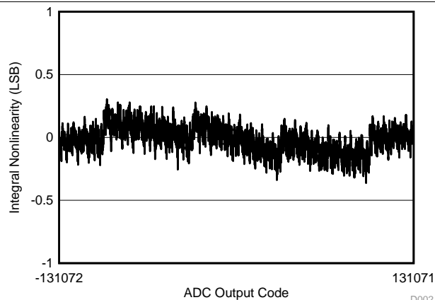
Figure 7. Typical INL
