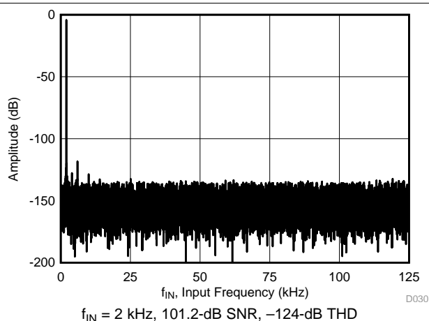
Figure 107. Noise-Performance FFT Plot - ADS8914B
