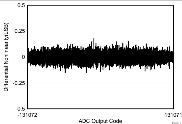
Figure 6. Typical DNL
