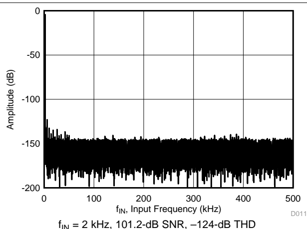
Figure 105. Noise-Performance FFT Plot - ADS8910B
