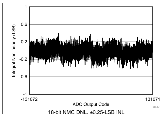
Figure 110. Typical Linearity, Differential Input
