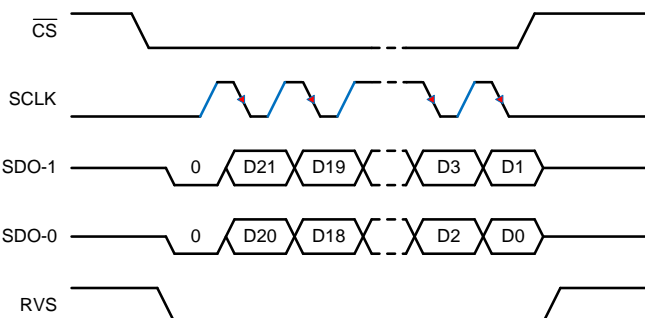
Figure 61. SPI-01-D Protocol
