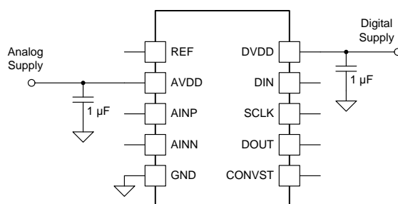
Figure 53. Supply Decoupling
