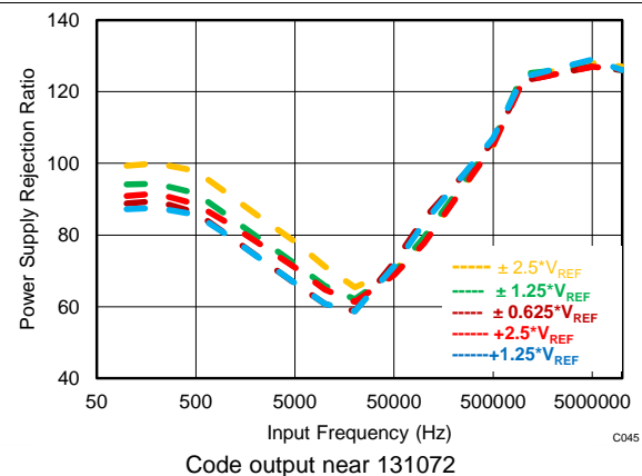
Figure 111. PSRR With a Decoupling Capacitor
