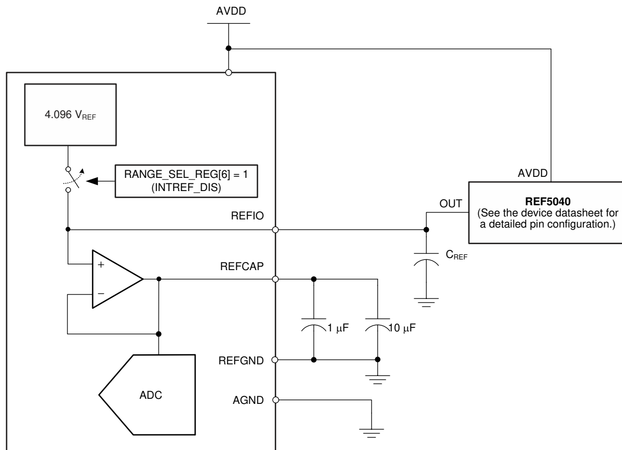
Figure 6-12. Device Connections for Using an External 4.096V Reference
