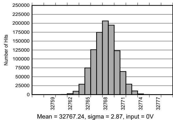
Figure 5-14. DC Histogram for Midscale Inputs (±10.24V)
