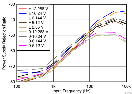
Figure 8-6. PSRR Without a Decoupling Capacitor
