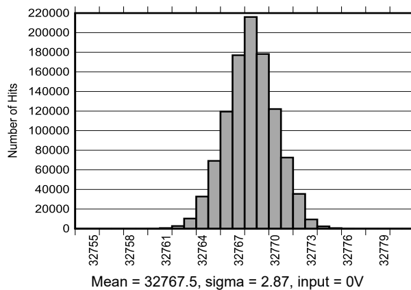
Figure 5-13. DC Histogram for Midscale Inputs (±12.288V)
