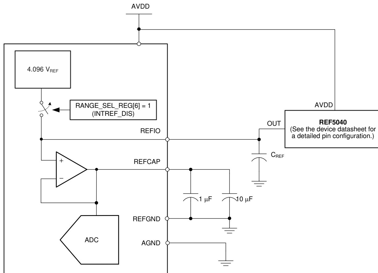
The output of the internal reference buffer appears at the REFCAP pin. A minimum capacitance of 10 \mu\text{F} must be placed between the REFCAP and REFGND pins. Place another capacitor of 1 \mu\text{F} as close to the REFCAP pin as possible for decoupling high-frequency signals. Do not use the internal buffer to drive external ac or dc loads because of the limited current output capability of this buffer.
