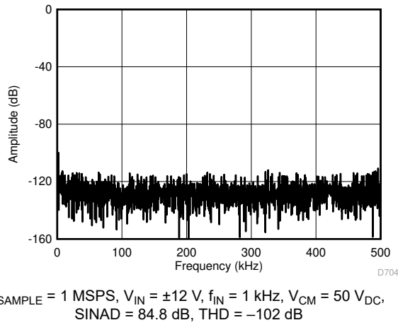
Figure 8-3. FFT Plot With a DC Common-Mode at 1 MSPS
