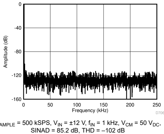
Figure 8-5. FFT Plot With a DC Common-Mode at 500 kSPS
