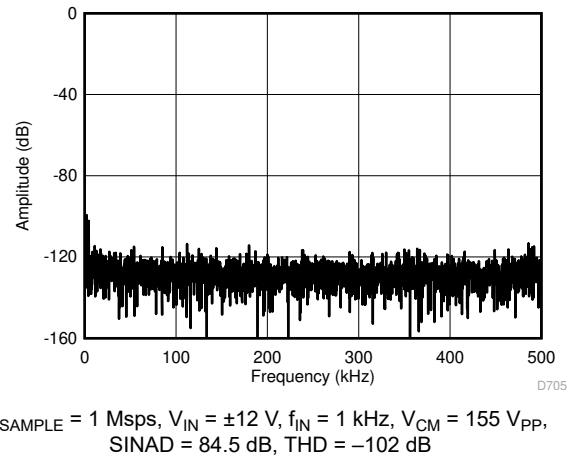
Figure 8-4. FFT Plot With an AC Common-Mode at 1 MSPS
