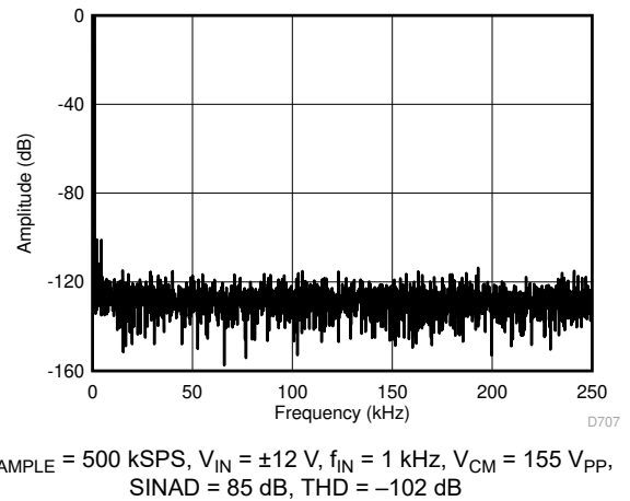
Figure 8-6. FFT Plot With an AC Common-Mode at 500 kSPS
