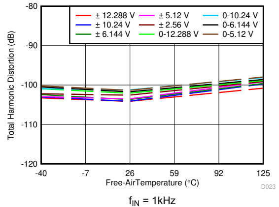
Figure 5-30. THD vs Temperature
