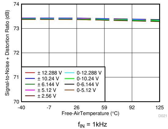
Figure 5-28. SINAD vs Temperature
