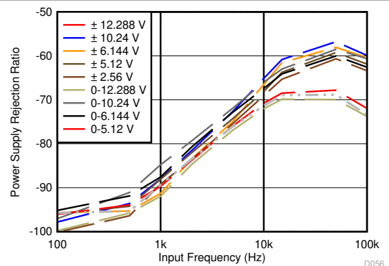
Figure 8-5. PSRR With a Decoupling Capacitor
