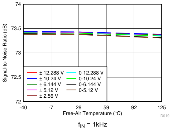
Figure 5-27. SNR vs Temperature
