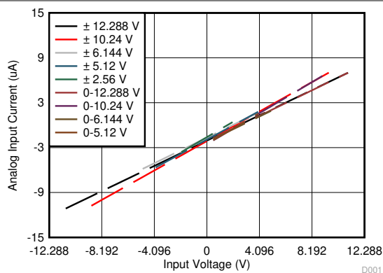
Figure 5-9. Input I-V Characteristic Across Input Ranges
