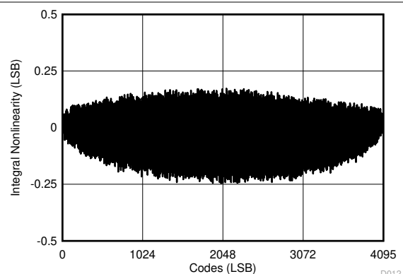
Figure 5-16. Typical INL for All Codes (All Bipolar Ranges)
