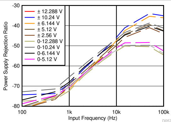
Figure 8-4. PSRR Without a Decoupling Capacitor
