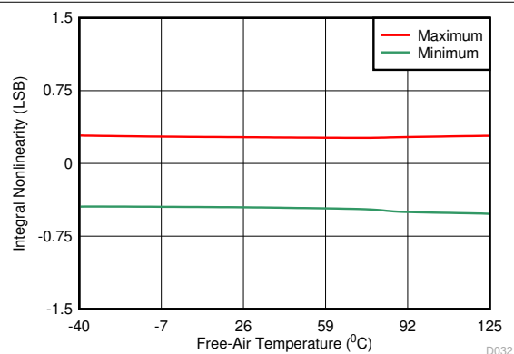
Figure 5-17. Typical INL for All Codes (All Unipolar Ranges)
