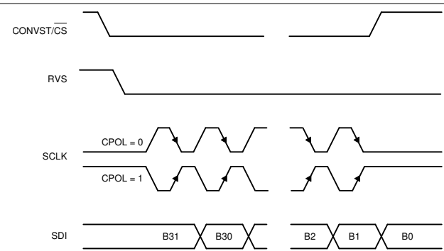
Figure 6-27. Standard SPI Timing Protocol (CPHA = 1, 32 SCLK Cycles)
