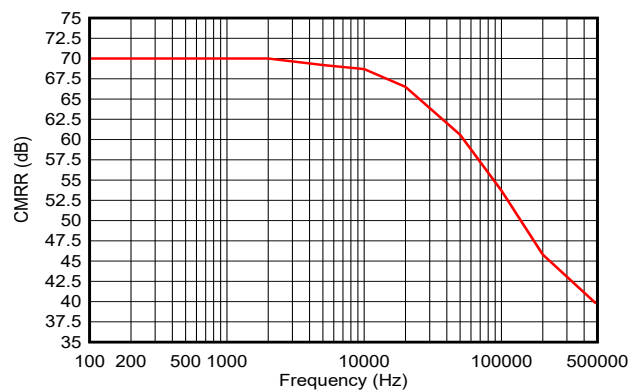
Figure 8-3. Common-Mode Rejection Ratio vs Frequency
