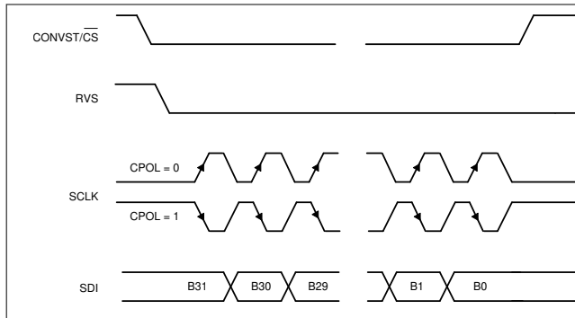
Figure 6-26. Standard SPI Timing Protocol (CPHA = 0, 32 SCLK Cycles)
