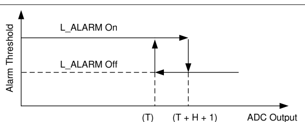
Figure 7-18. Low ALARM Hysteresis
