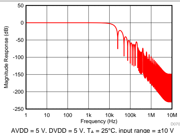
Figure 80. Digital Filter Response for OSR = 8
