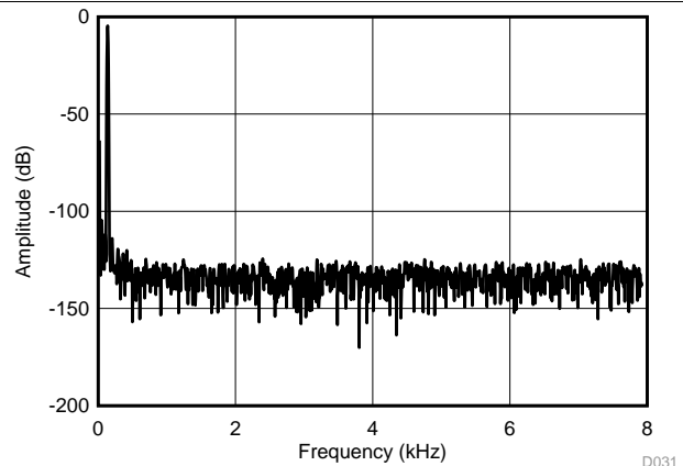
Figure 35. Typical FFT Plot for OSR 32x (±5 V)
