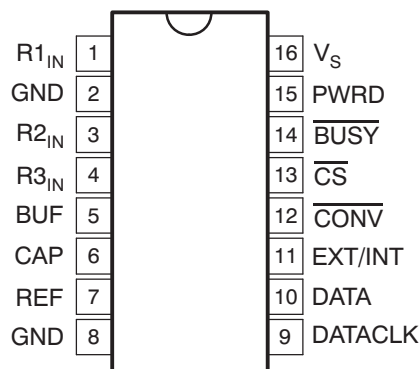
DW PACKAGE SO-16 (TOP VIEW)
