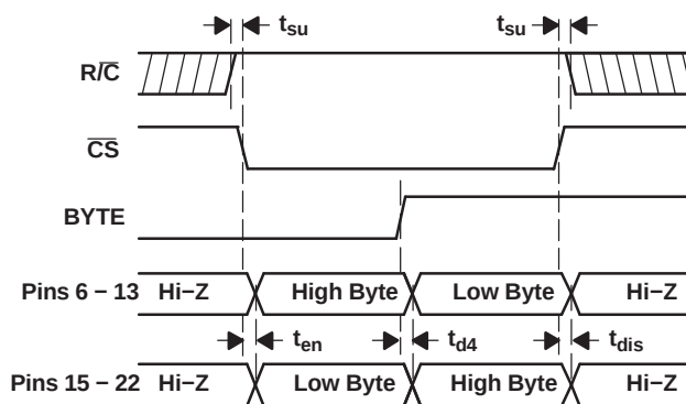
Figure 25. Using \overline{\text{CS}} and \overline{\text{BYTE}} to Control Data Bus
