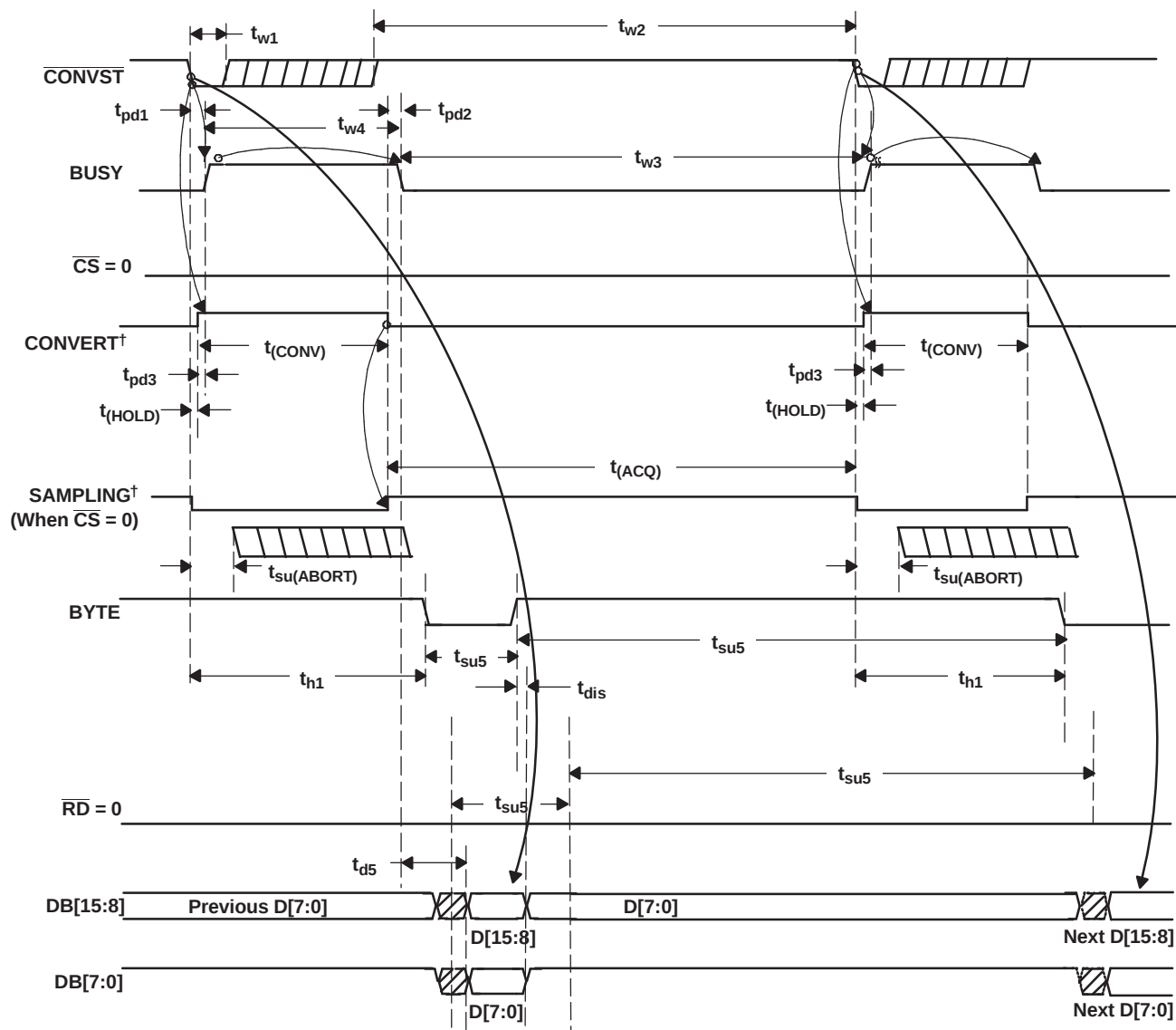
Figure 34. Timing for Conversion and Acquisition Cycles With \overline{\text{CS}} and \overline{\text{RD}} Tied to BDGND - Auto Read
