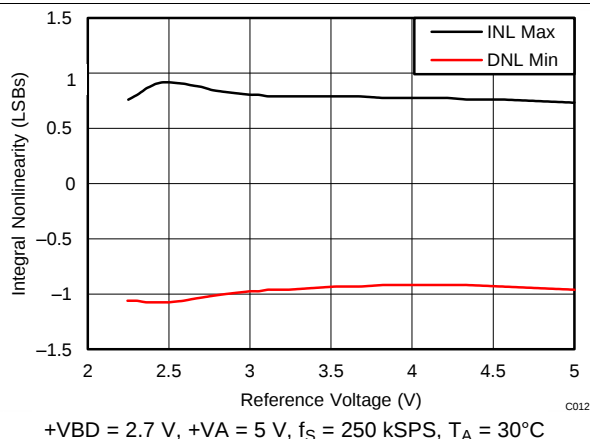
Figure 12. INL vs Reference Voltage
