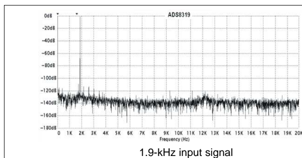
Figure 62. FFT
