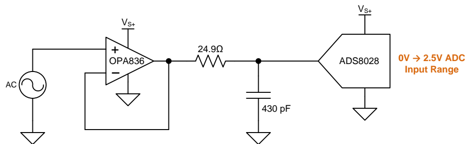
Figure 40. OPA836 Buffer
