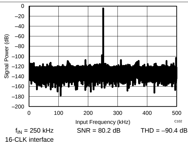
Figure 25. Typical FFT
