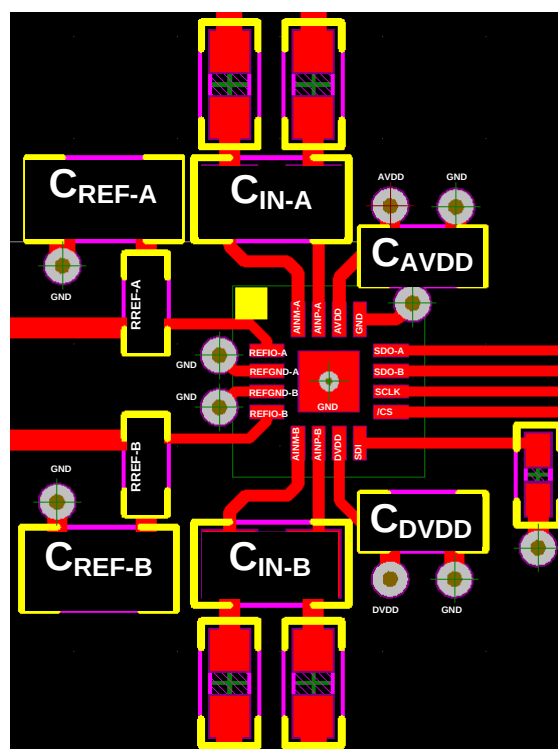
Figure 117. Recommended Layout
