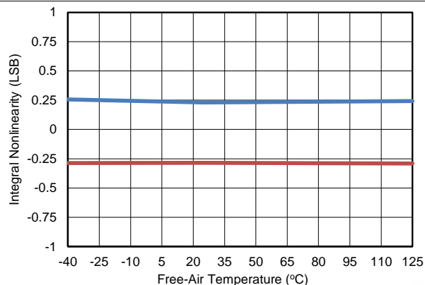
Figure 12. Typical INL
