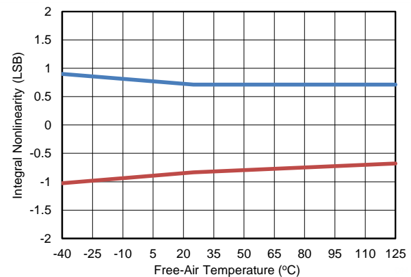
Figure 28. Typical INL
