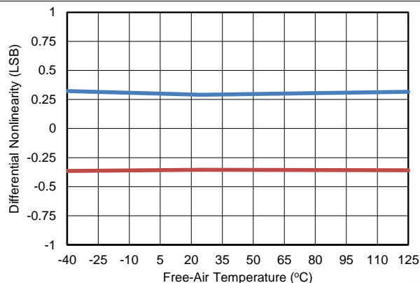
Figure 11. Typical DNL
