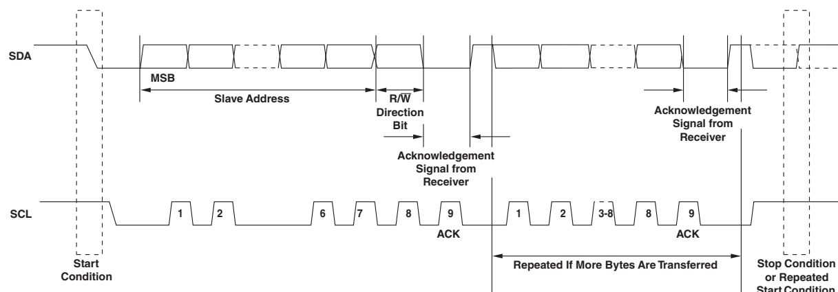
Figure 14. Basic Operation
