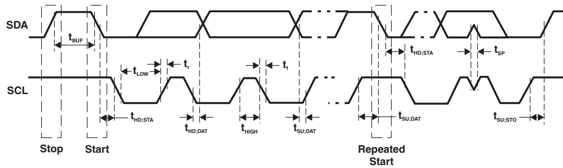
Figure 1. I²C Timing
