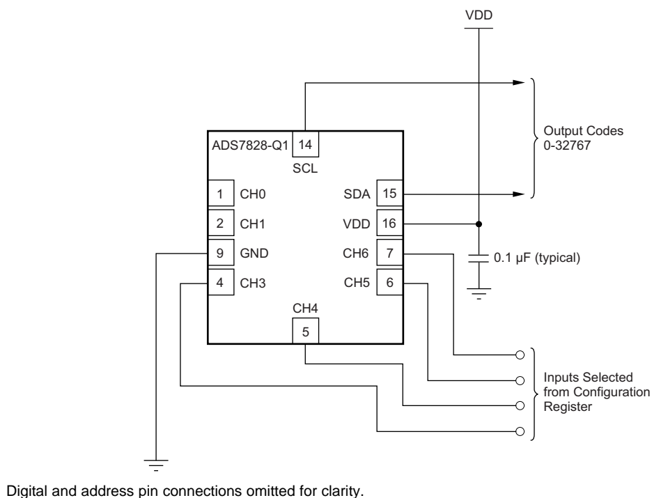
Figure 24. Measuring Single-Ended Inputs
