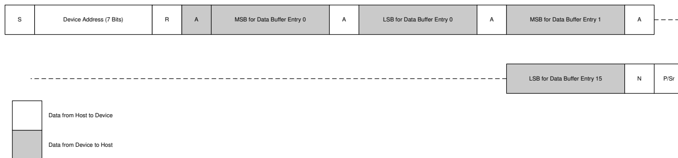
Figure 7-8. Reading Data Buffer (16 Bit Words x 16 Words)
