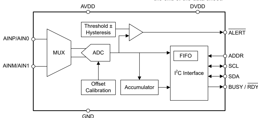
Block Diagram
