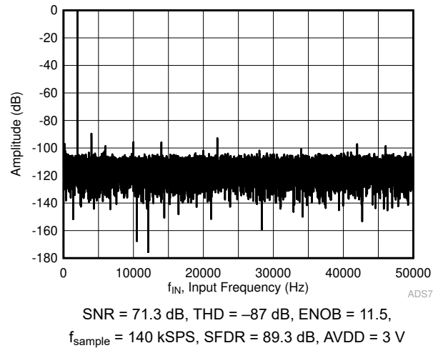
Figure 6-6. Typical FFT in Manual Mode
