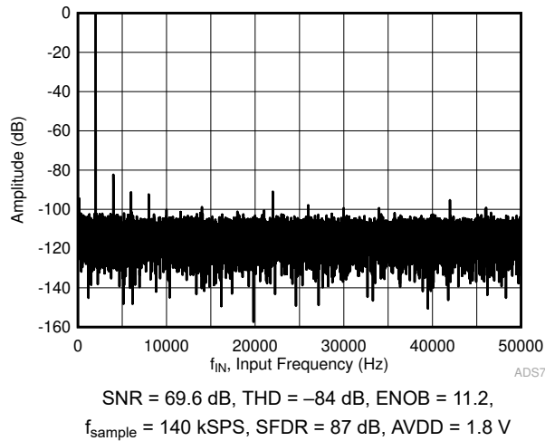
Figure 6-5. Typical FFT in Manual Mode
